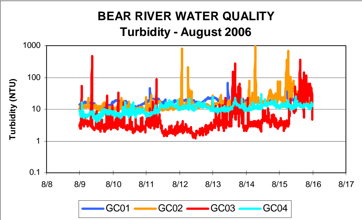
Figure 3-10. Turbidity at four monitoring stations during August 2006.
