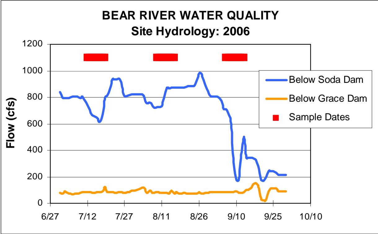
Figure 3-1. Flows recorded in the Bear River during the 2006 monitoring period.
