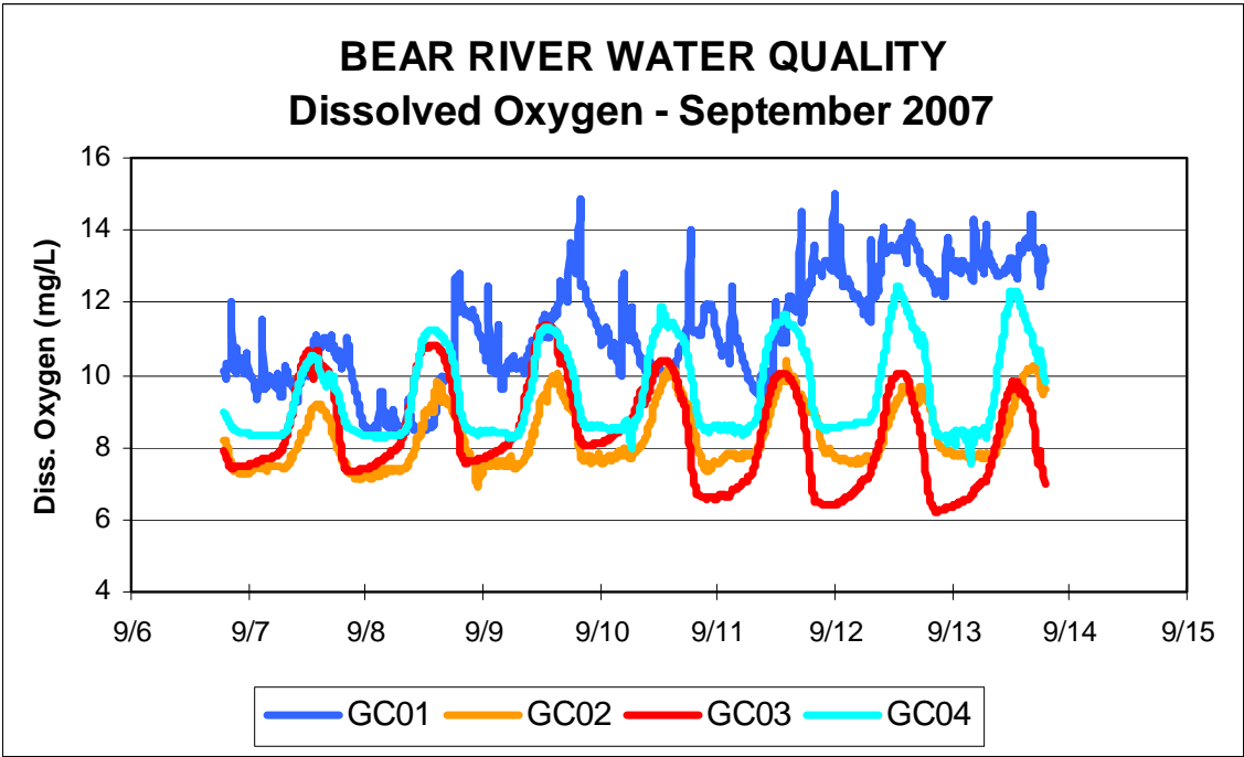
Figure 21. Dissolved oxygen (mg/L) at the four monitoring locations during September 2007.
