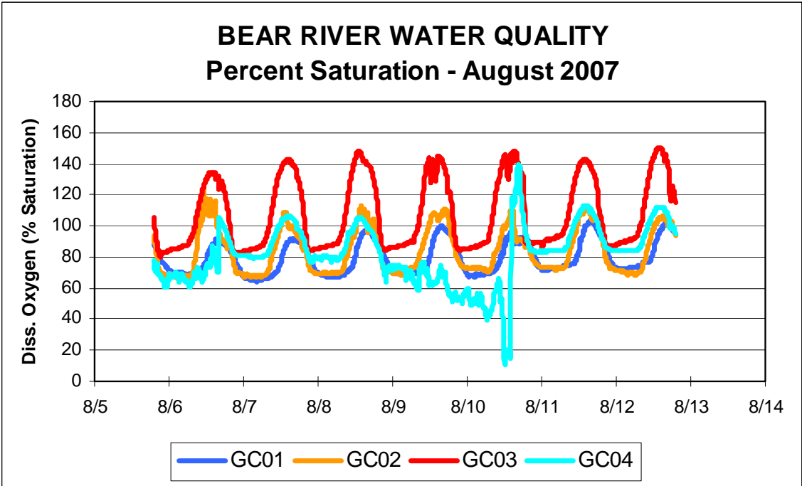
Figure 17. Dissolved oxygen (% saturation) at the four monitoring locations during August 2007.
