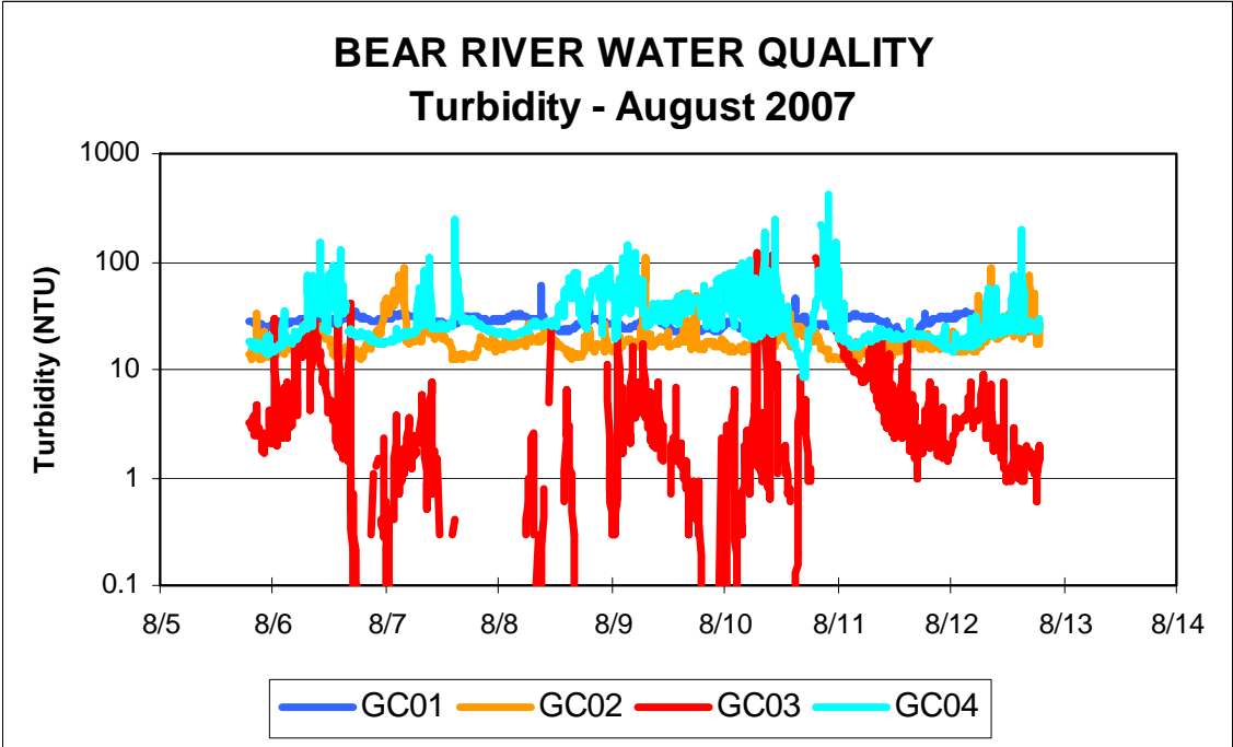
Figure 18. Turbidity at the four monitoring locations during August 2007.
