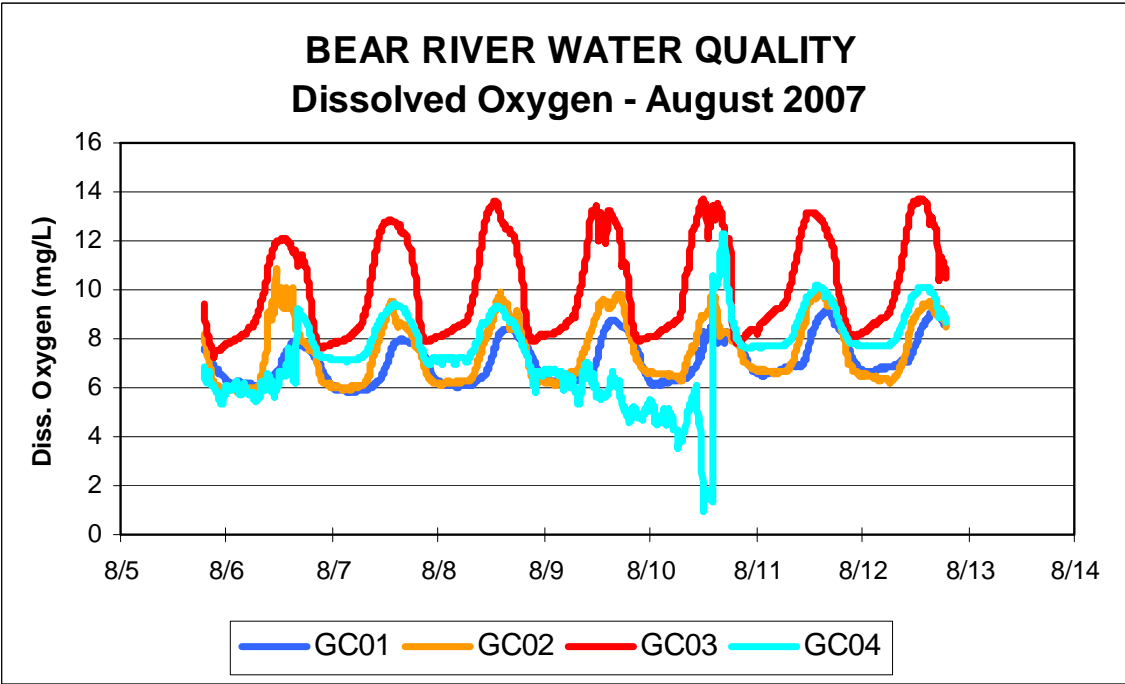
Figure 16. Dissolved oxygen (mg/L) at the four monitoring locations during August 2007.
