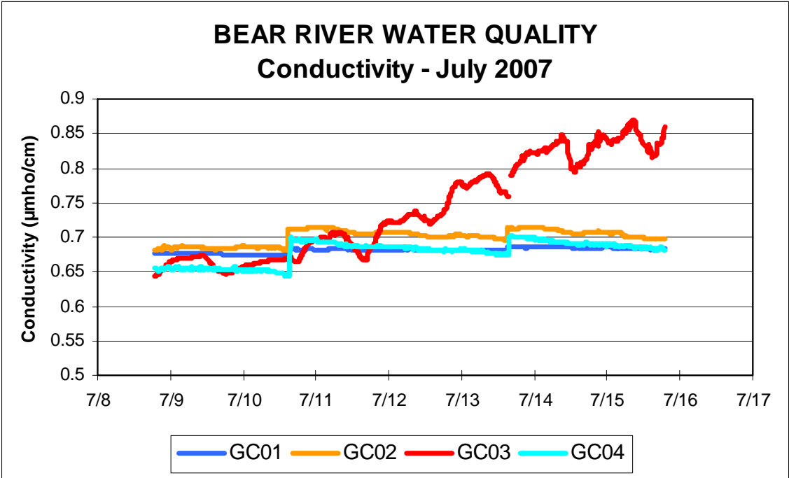
Figure 14. Specific conductance at the four monitoring locations during July 2007.
