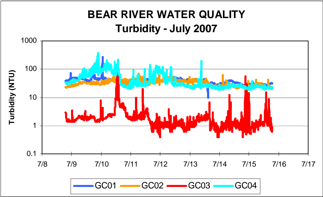
Figure 13. Turbidity at the four monitoring locations during July 2007.
