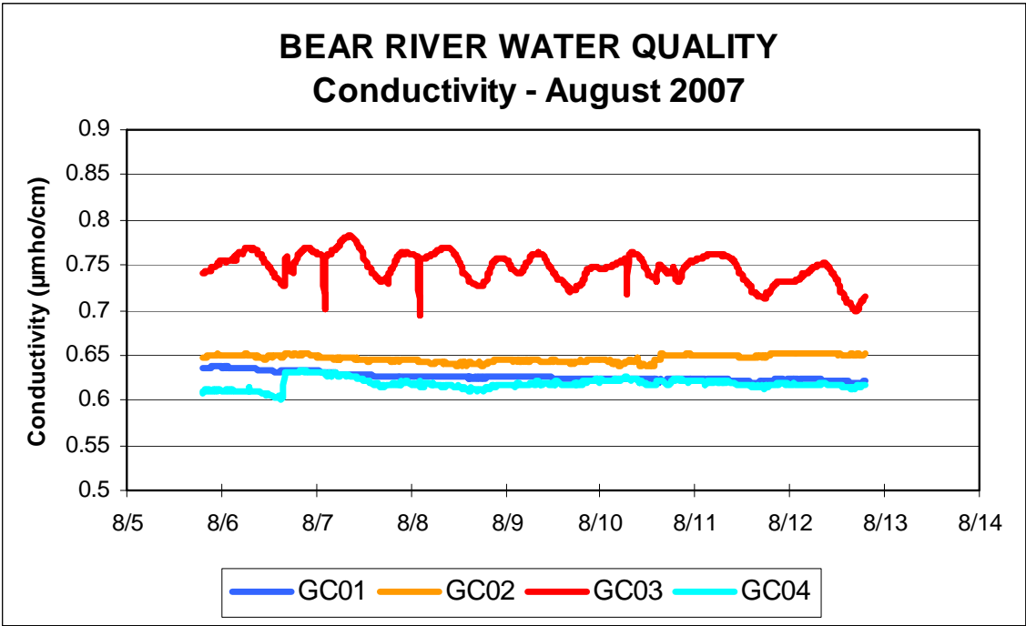
Figure 19. Specific conductance at the four monitoring locations during August 2007.
