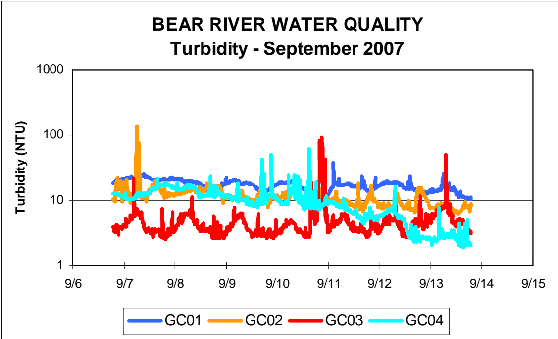
Figure 23. Turbidity at the four monitoring locations during September 2007.
