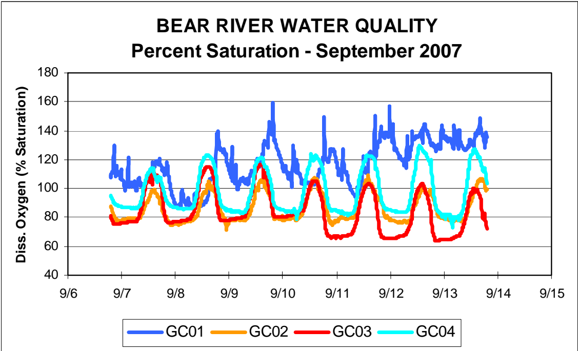
Figure 22. Dissolved oxygen (% saturation) at the four monitoring locations during September 2007.
