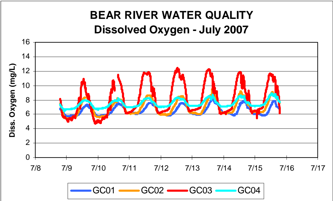
Figure 11. Dissolved oxygen (mg/L) at the four monitoring locations during July 2007.
