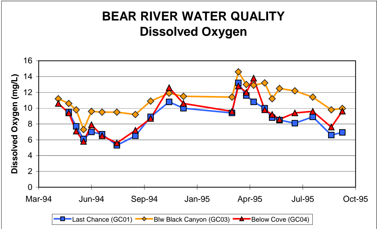
Figure 2. The dissolved oxygen concentrations at five locations in the Bear River above Cove from 1994-1996.
