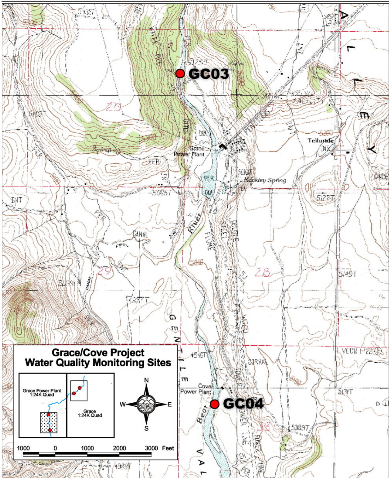
Figure 8. The location of the lowermost monitoring sites for the Grace/Cove WQMP.
