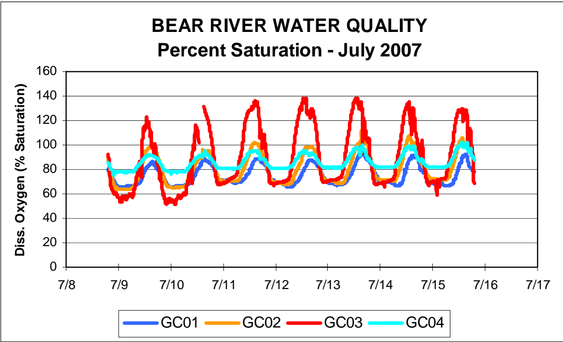
Figure 12. Dissolved oxygen (% saturation) at the four monitoring locations during July 2007.
