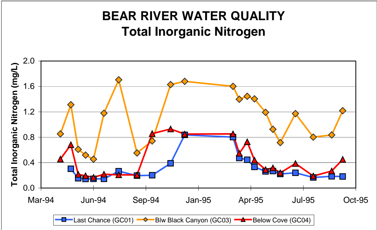
Figure 6. The total inorganic nitrogen concentrations at five locations in the Bear River above Cove from 1994-1996.
