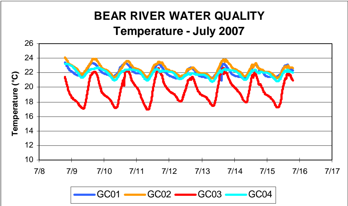
Figure 10. Temperature at the four monitoring locations during July 2007.
