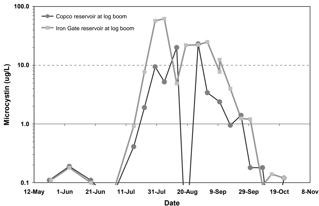
Figure 3. Microcystin data obtained in water samples from the surface waters over the deepest part (near the log boom) in Copco and Iron Gate reservoirs, May to November 2008. Note that the y-axis is logarithmic in scale.
