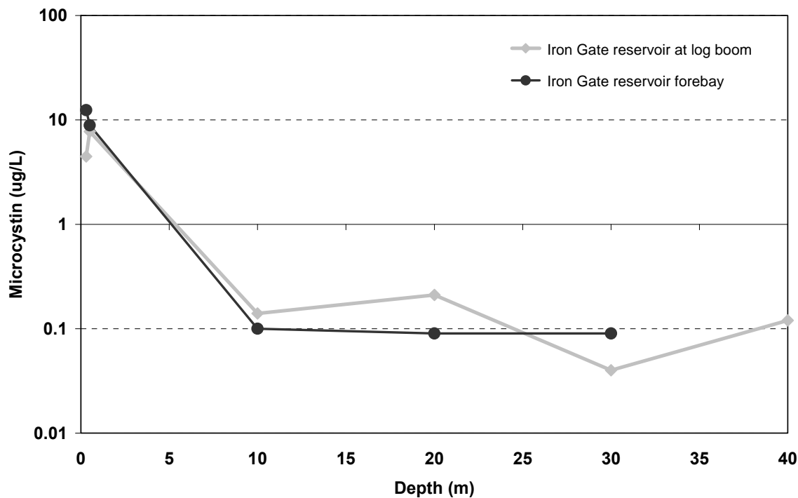
Figure 5. Data obtained on September 10, 2008 to assess in-water concentrations of microcystin at various depths in Iron Gate reservoir in the forebay and near the log boom. Note that the y-axis is logarithmic in scale.
