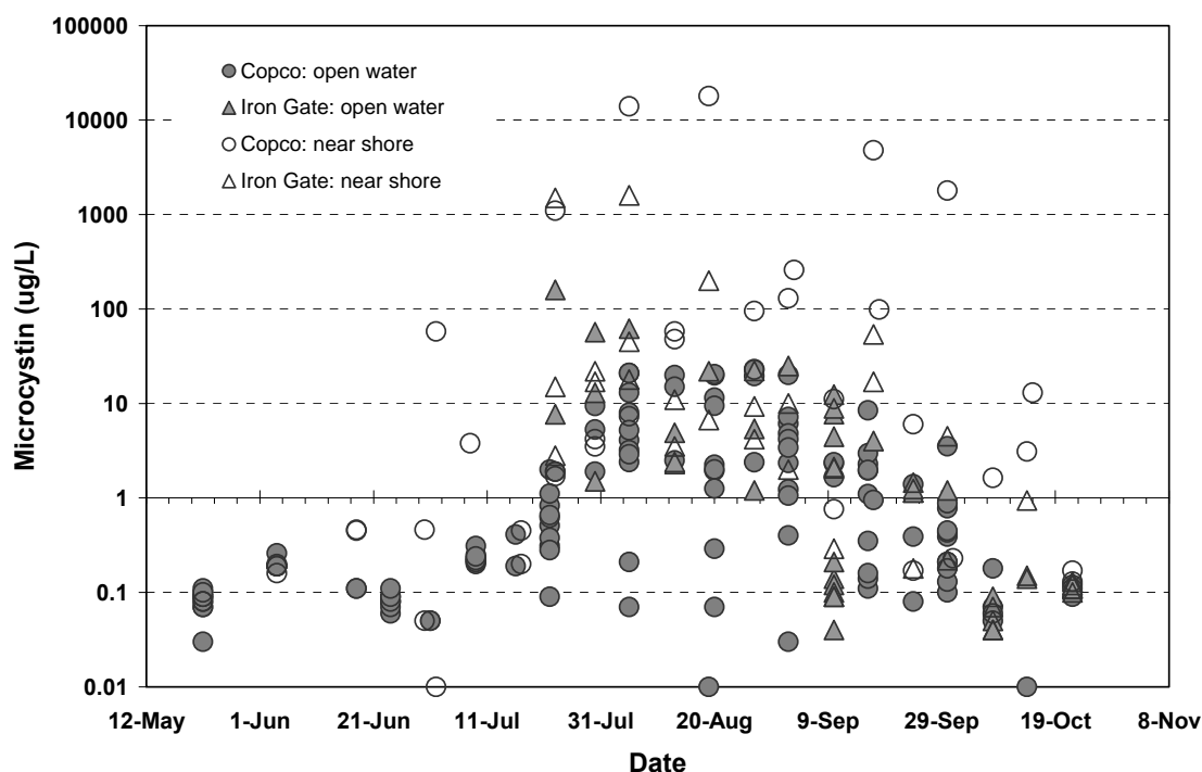
Figure 4. Microcystin data obtained in water samples from shoreline and open water locations throughout both Copco and Iron Gate reservoirs. May to November 2008. Note that the y-axis is logarithmic in scale.
