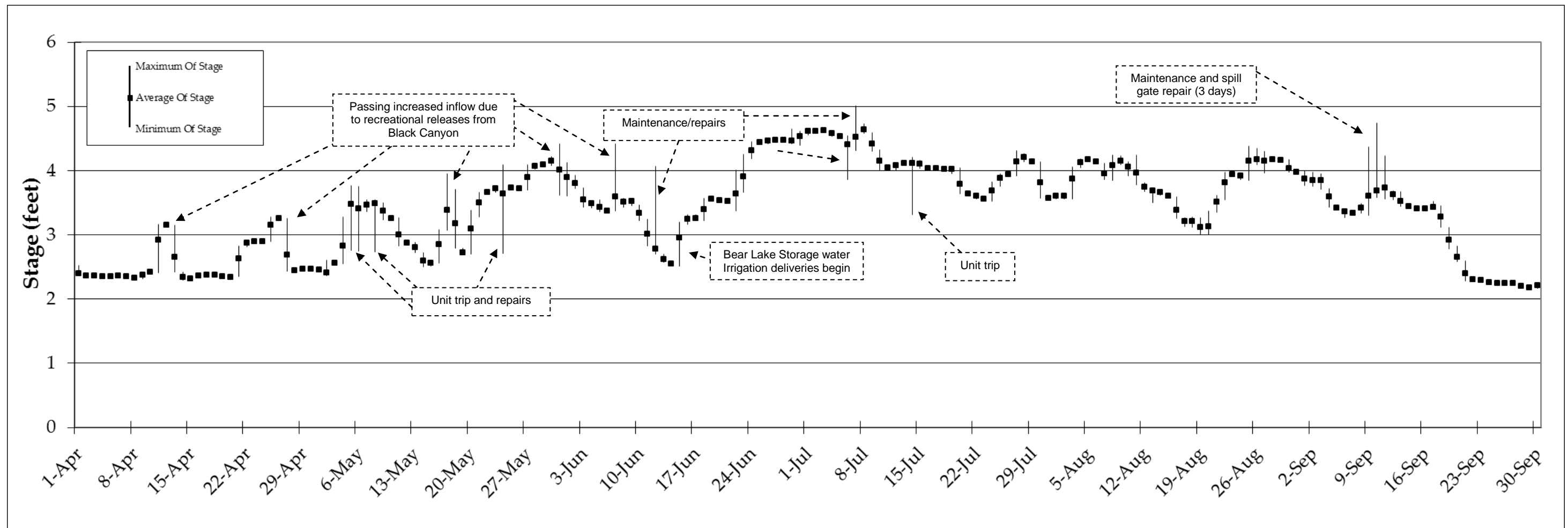
Figure 4. April through September 2015 daily average, maximum and minimum stage below Oneida. Precise values for each day and explanations are provided in Appendix A. Corresponding power releases are shown in Figure 1.
