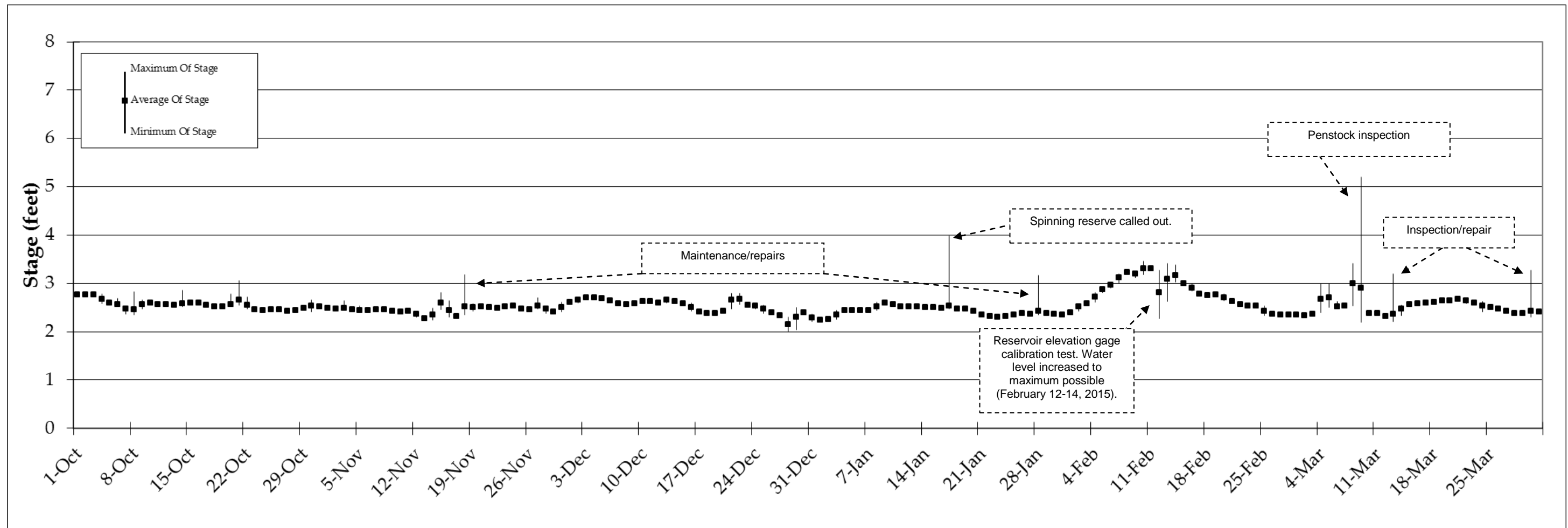
Figure 3. October 2014 through March 2015 daily average, maximum and minimum stage below Oneida. Precise values for each day and explanations are provided in Appendix A. Corresponding flows are shown in Figure 1.
