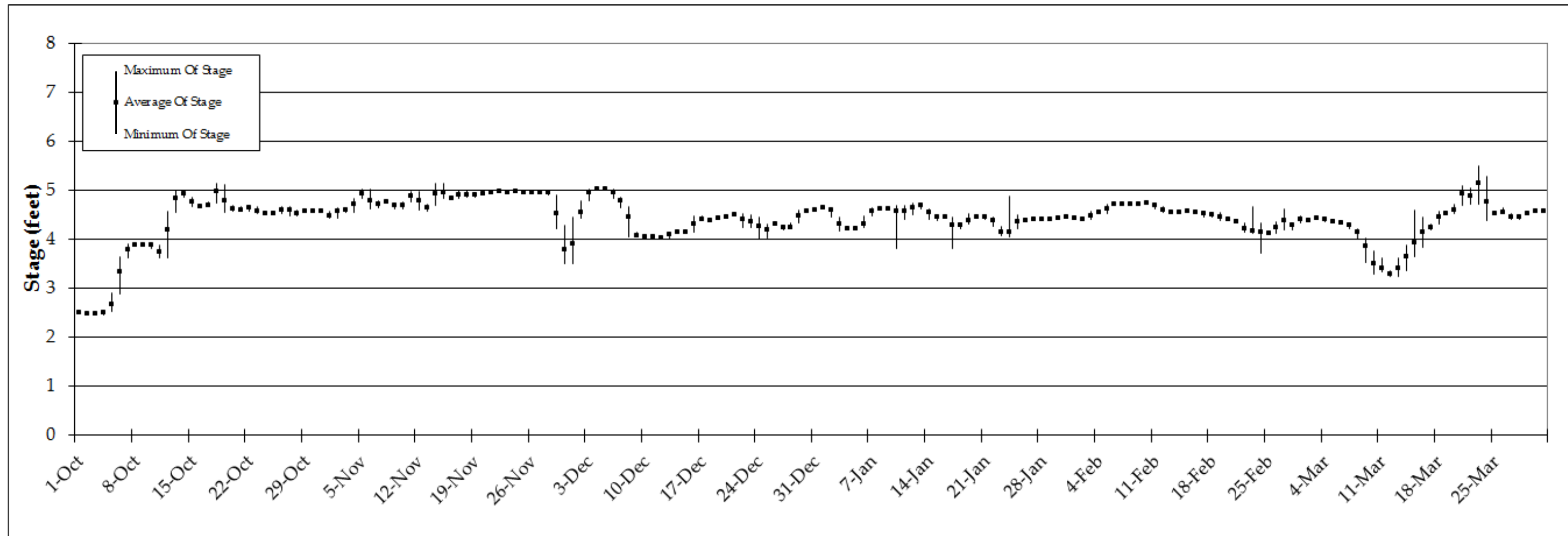
Figure 3. October 2017 through March 2018 daily average, maximum and minimum stage below Oneida. Precise values for each day and explanations are provided in Appendix A. Corresponding flows are shown in Figure 1.
