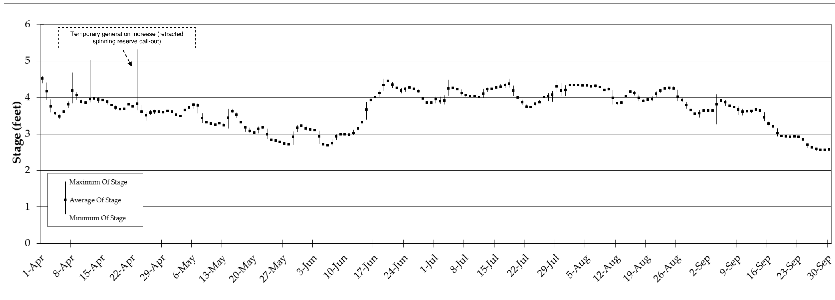
Figure 4. April through September 2018 daily average, maximum and minimum stage below Oneida. Precise values for each day and explanations are provided in Appendix A. Corresponding power releases are shown in Figure 1.
