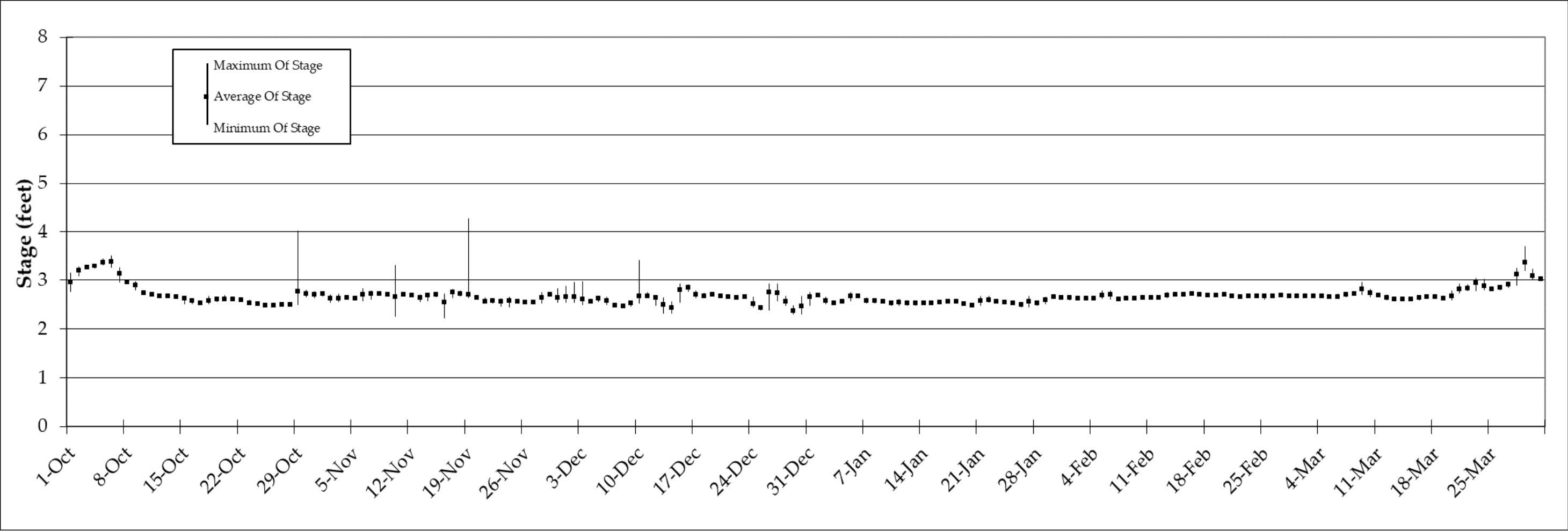
Figure 3. October 2020 through March 2021 daily average, maximum and minimum stage below Oneida. Precise values for each day and explanations are provided in Appendix A. Corresponding flows are shown in Figure 1.
