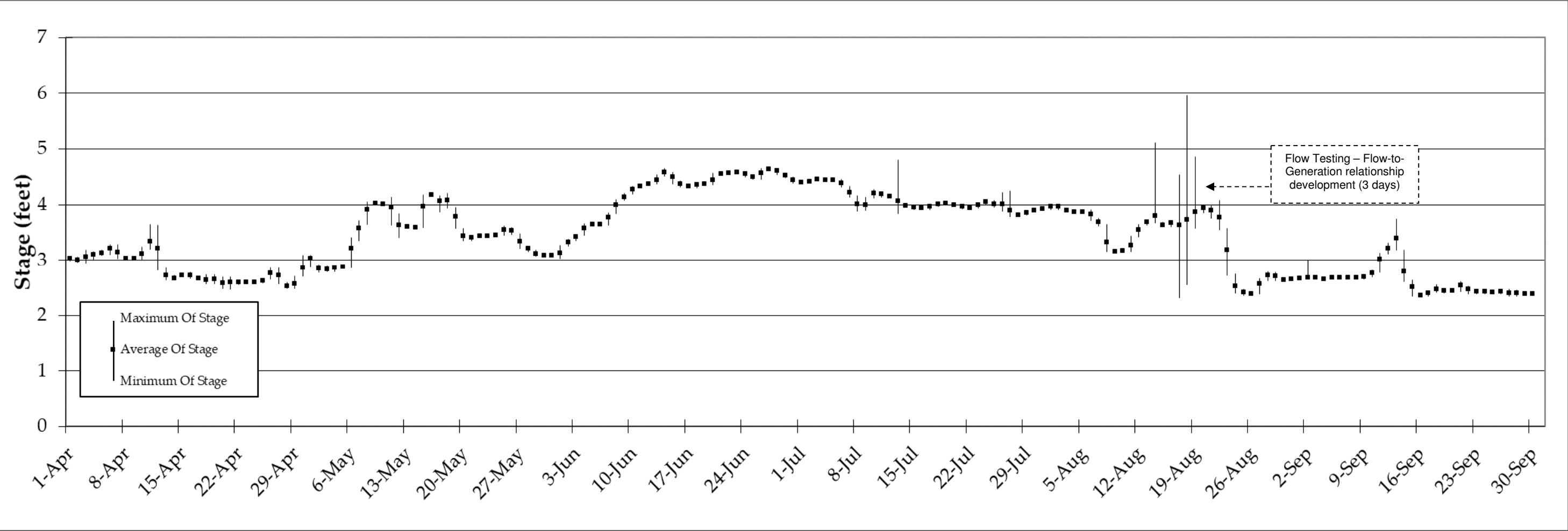
Figure 4. April through September 2021 daily average, maximum and minimum stage below Oneida. Precise values for each day and explanations are provided in Appendix A. Corresponding power releases are shown in Figure 1.
