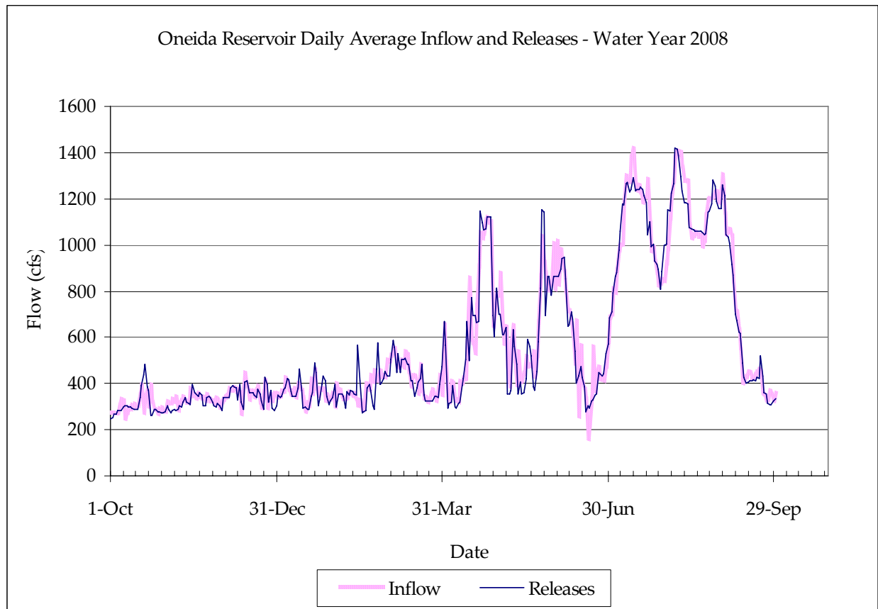
Figure 1. Daily average reservoir inflow and releases (no significant spill flow). Flows are in cubic feet per second (CFS).
