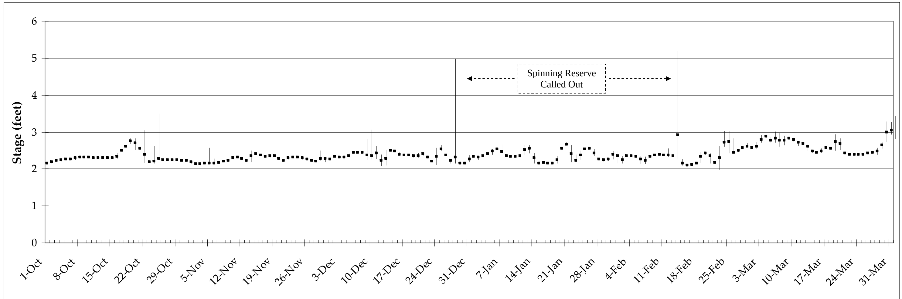
Figure 3. October 2007 through March 2008 daily average, maximum and minimum stage below Oneida. Precise values for each day and explanations are provided in Appendix A. Corresponding flows are shown in Figure 1.
