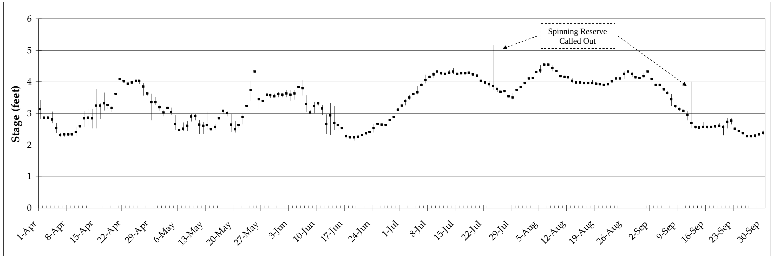
Figure 4. April through September 2008 daily average, maximum and minimum stage below Oneida. Precise values for each day and explanations are provided in Appendix A. Corresponding flows are shown in Figure 1.
