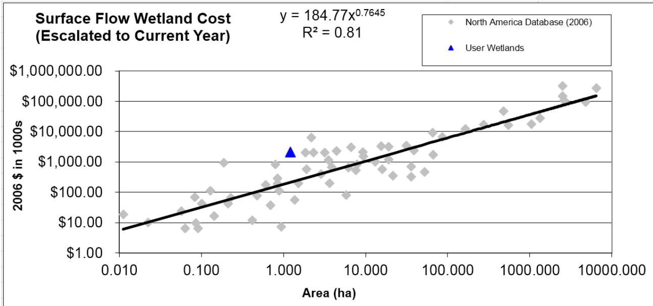
FIGURE 4-9 Surface Flow Wetland Cost Graph
