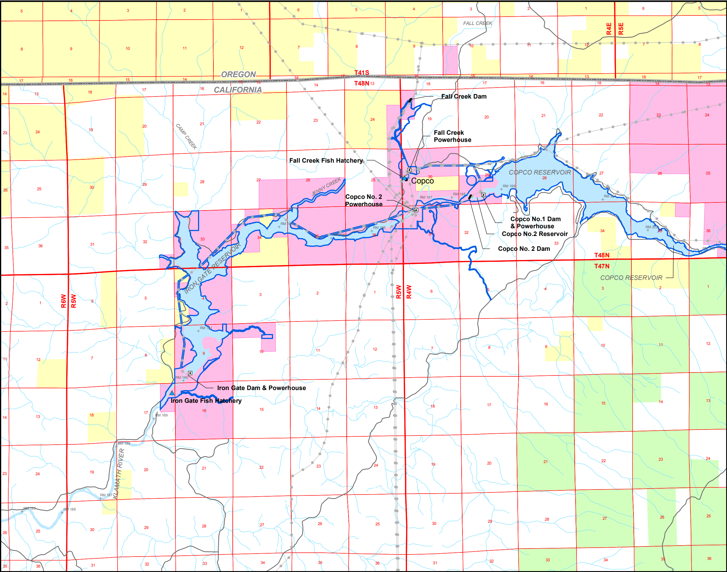
Klamath Hydroelectric Project Figure 2.4-1 (4 of 4) Project Area
