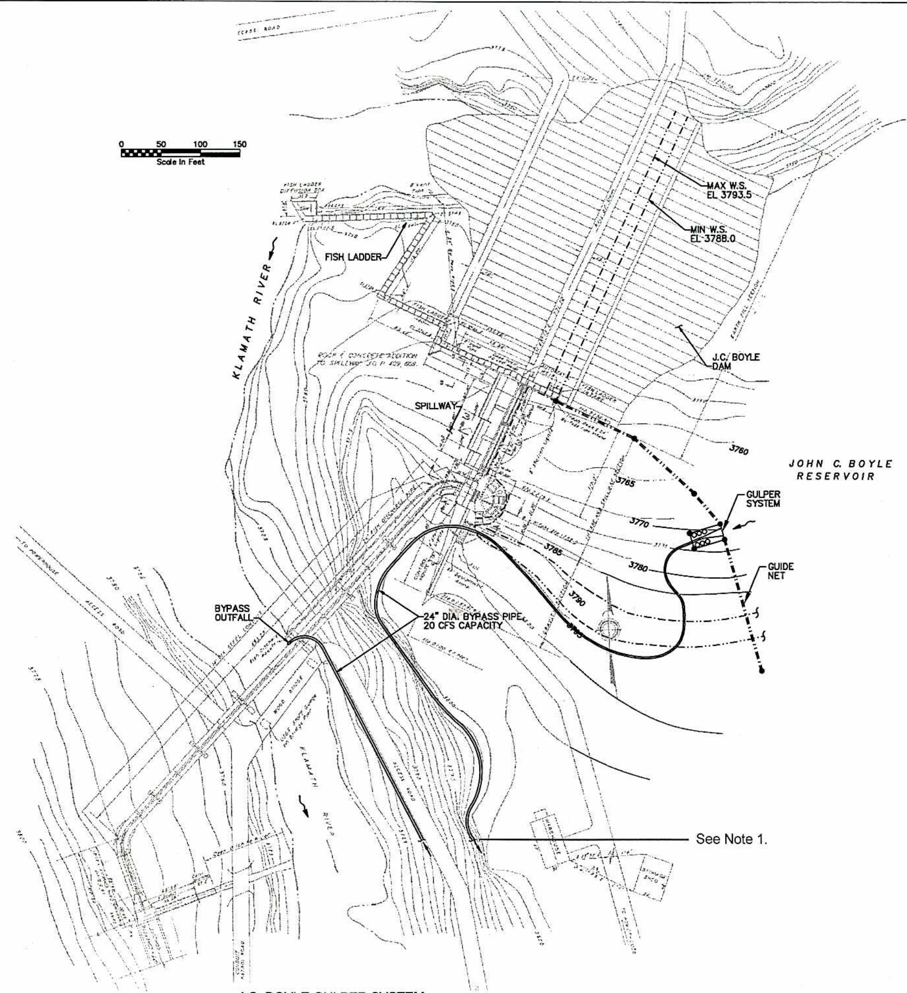
J.C. BOYLE GULPER SYSTEM 1" = 50'-0"
