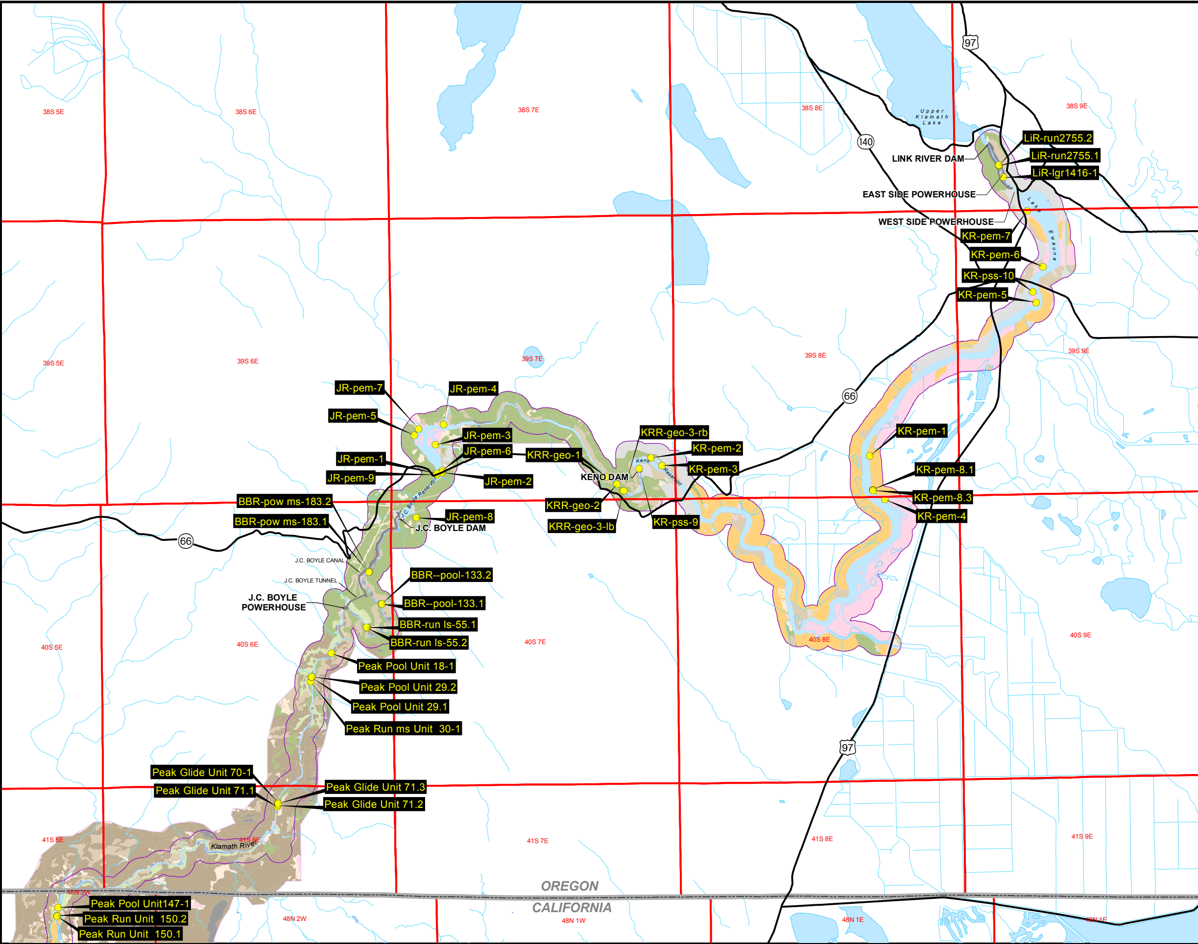
Klamath Hydroelectric Project Figure 3.7-1 (1 of 2) Riparian Sampling Locations
