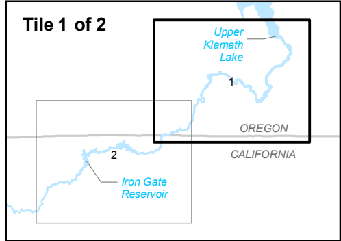
Klamath Hydroelectric Project Figure 3.7-1 (1 of 2) Riparian Sampling Locations
