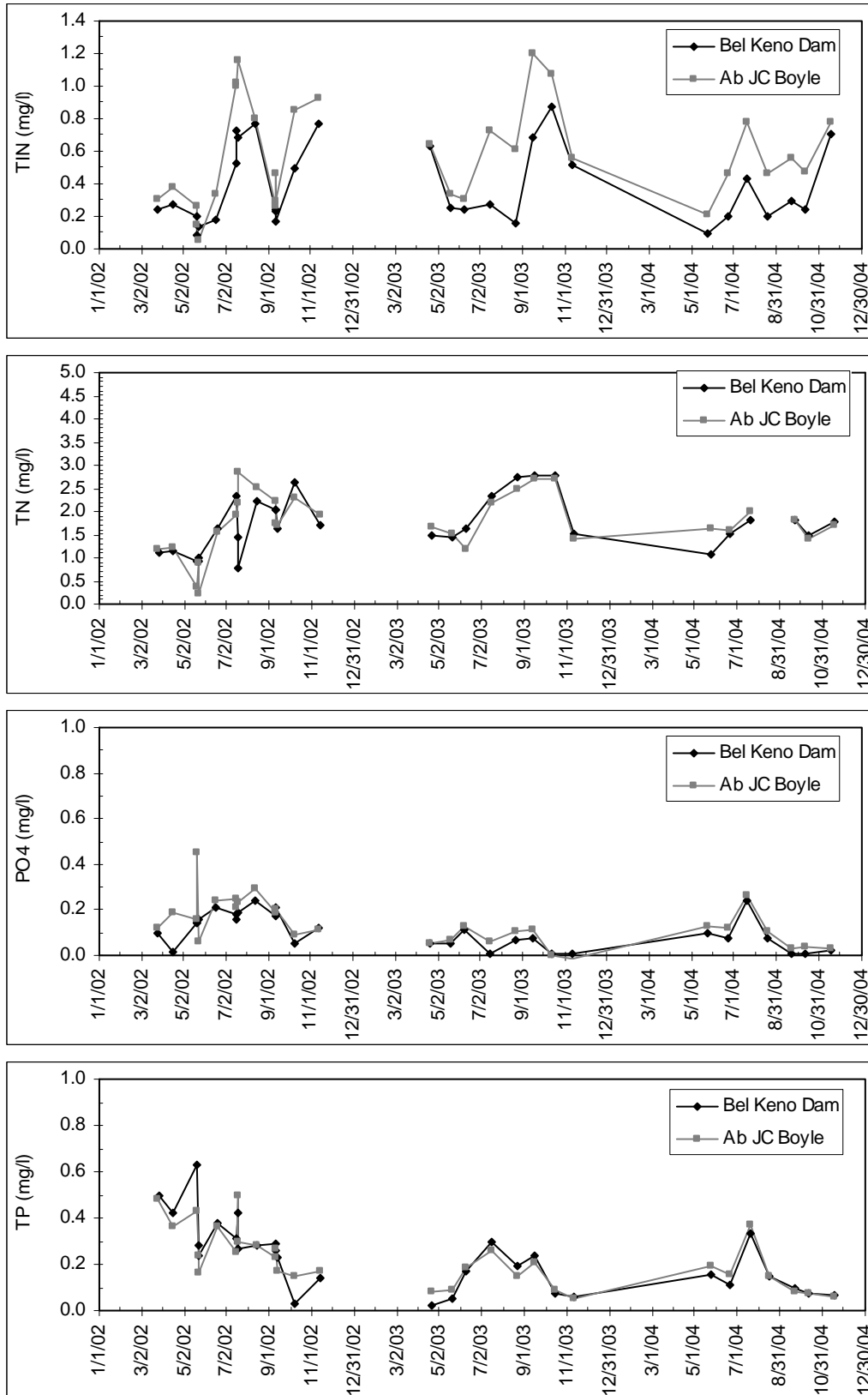
Figure 4-8. Observed total inorganic nitrogen (TIN), total nitrogen (TN), orthophosphate (PO4), and total phosphorus (TP) in the upper and lower end of Keno reach, 2002-2004.
