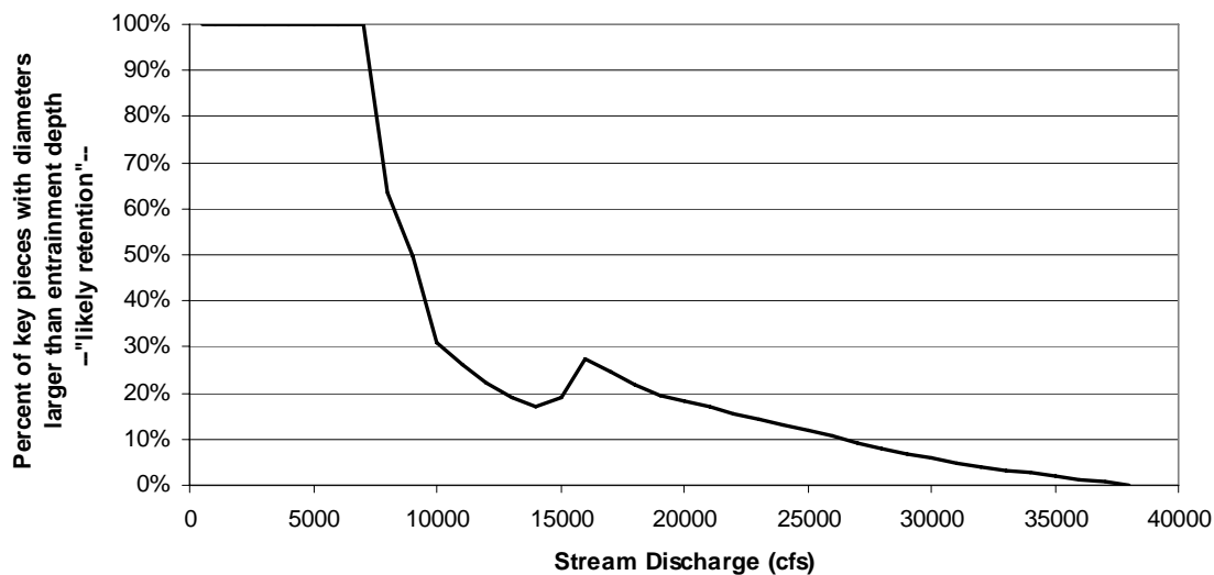
Figure 6. The percent of key pieces ( >10.75 \text{ m}^3 ) (based on current basin supply) with diameters larger than entrainment depth at a range of flows. Typical riffle cross section at river mile 13.6. Retention (the opposite of entrainment) is assumed when piece diameter exceeds 0.6 of the average flow depth across the cross section (based on Braudrick and Grant 2000). The spike in retention potential beginning at 14,000 cfs is due to overtopping of the floodplain terrace, which increases the amount of shallow depth area across the cross-section.
