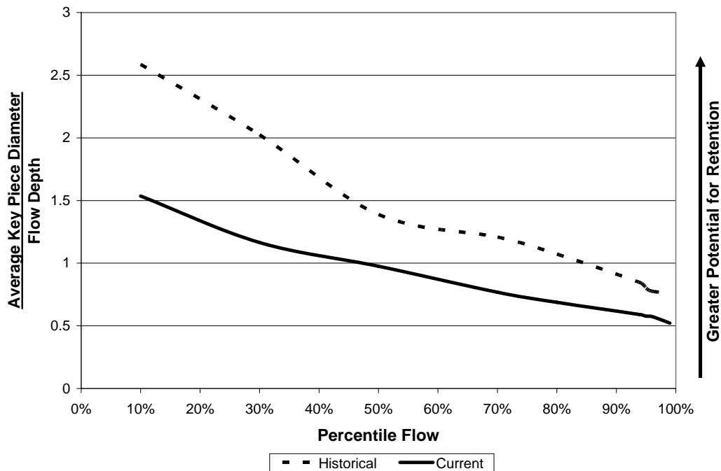
Figure 8. Ratio of average piece diameter to average flow depth plotted against flow for the historical and existing conditions. As flow depth decreases with respect to piece diameter, the potential for retention in the channel increases. Historical and current average piece diameters are 1.5 and 1.1 meters, respectively. Percentile flow is used because the flow regime is different for the historical (pre-Merwin Dam) and existing (last 30-years) condition. Percentile flow is the percentile flow using all average daily flows for the period (historical = Aug 1923 – July 1930; existing = Sept 1978 – Aug 2007). Thus, the 50% flow represents the median flow for the period and the 100% flow represents the greatest flow for the period.
