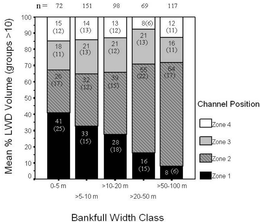
Figure 2. Comparison of the mean percent LWD volume by four lateral zone distributions according to five bank-full width classes. Only groups (accumulations) exceeding 10 pieces LWD are included. Zone 1 is the wetted low-flow channel, Zone 2 is above the wetted low-flow channel but below the horizontal axis of the bank-full channel, Zone 3 is above the high-flow channel but within the vertical confines of bank-full, and Zone 4 is laterally beyond the bank-full width. Zone definitions are from Schuett-Hames (1999). The numbers in parentheses are the standard deviations, and n = the number of LWD groups. Source: Fox (2003).
