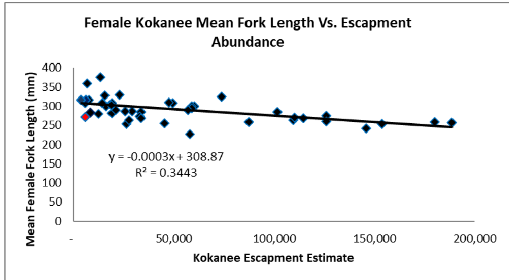
Figure 4. Relationship between mean kokanee fork length (female) and spawning escapement in Cougar Creek (1978-2022). Red dot represents year 2022, black dots are all other years on record.
