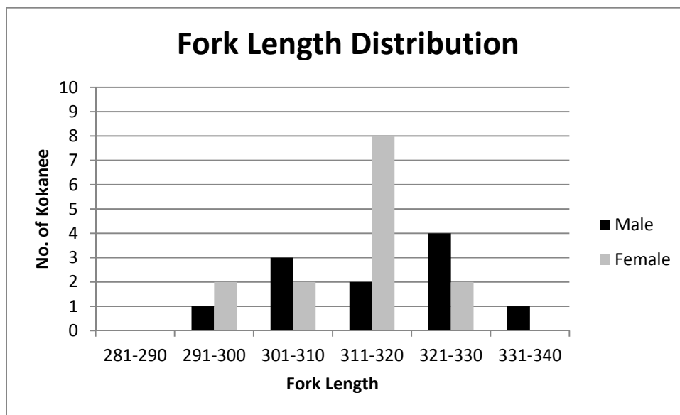
Figure 3. Length frequency histogram of male (n=11) and female (n=14) kokanee lengths (FL) sampled in Cougar Creek and the Constructed Channel, Washington – 2018
