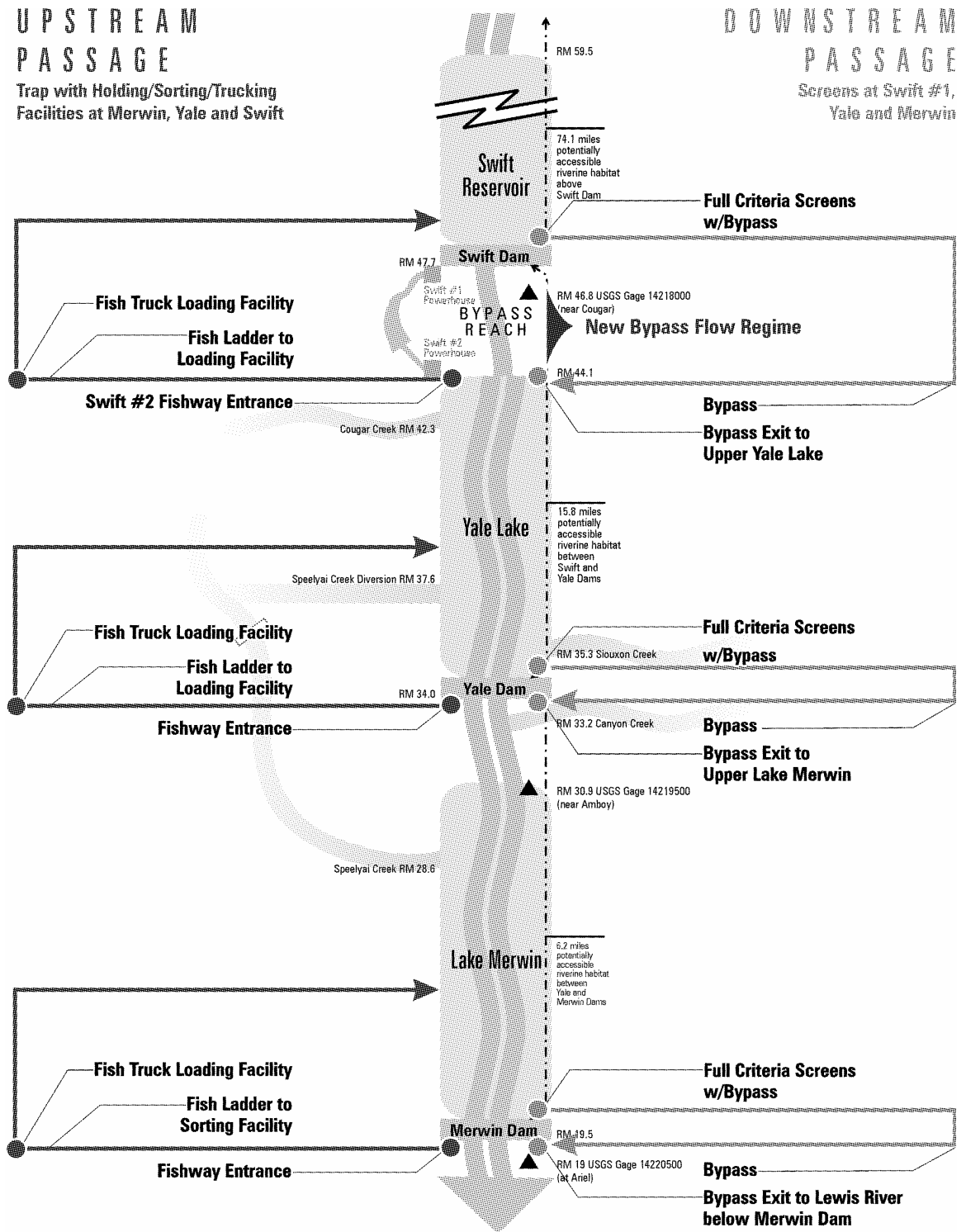
Figure 4.5-7. System 7: Resident trap-and-haul (no anadromous reintroduction).
