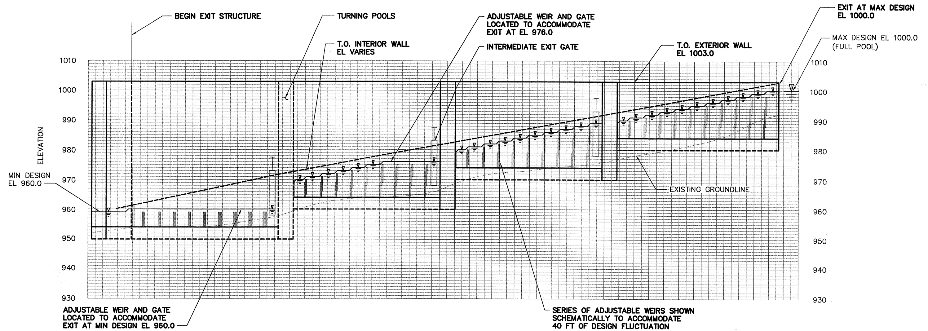
EXIT STRUCTURE ELEVATION
