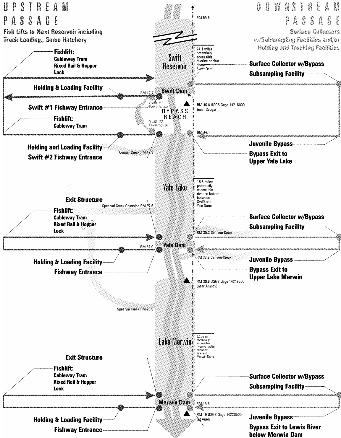
Figure 4.5-4. System 4: Fish lifts upstream, surface collectors downstream with trucking facilities.
