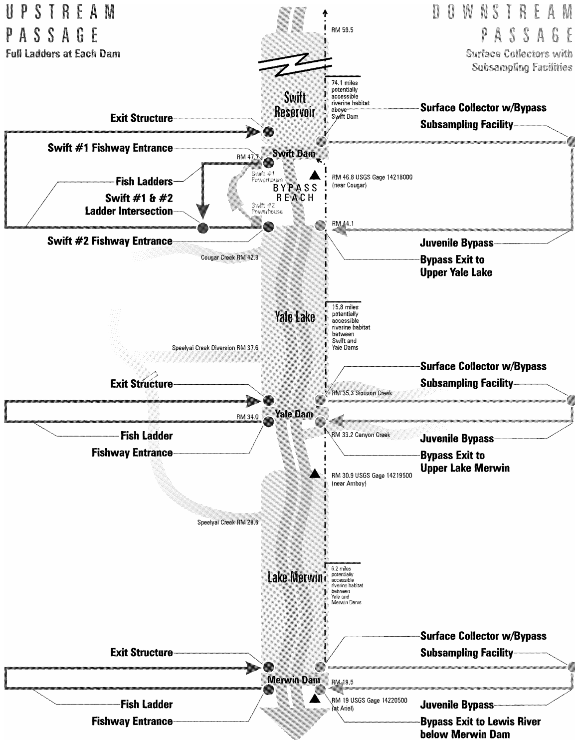
Figure 4.5-2. System 2: Volitional passage with surface collectors.
