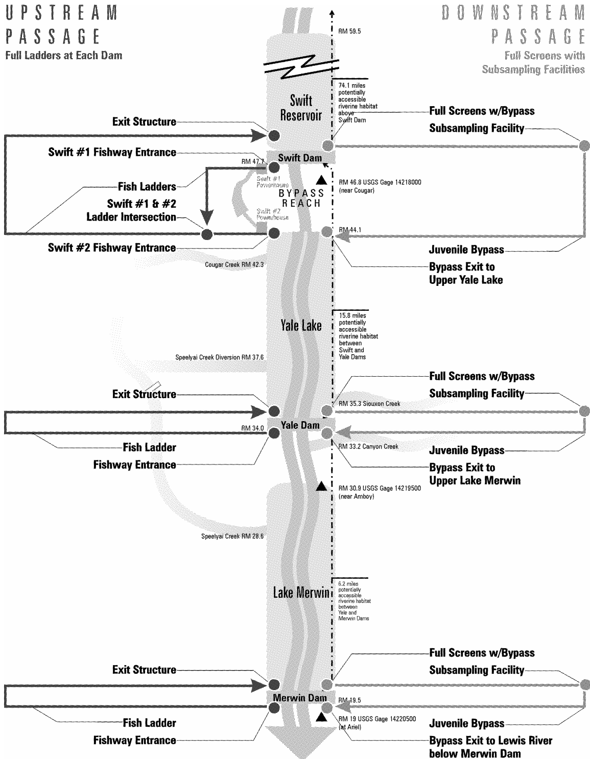
Figure 4.5-1. System 1: Volitional passage with criteria screens.
