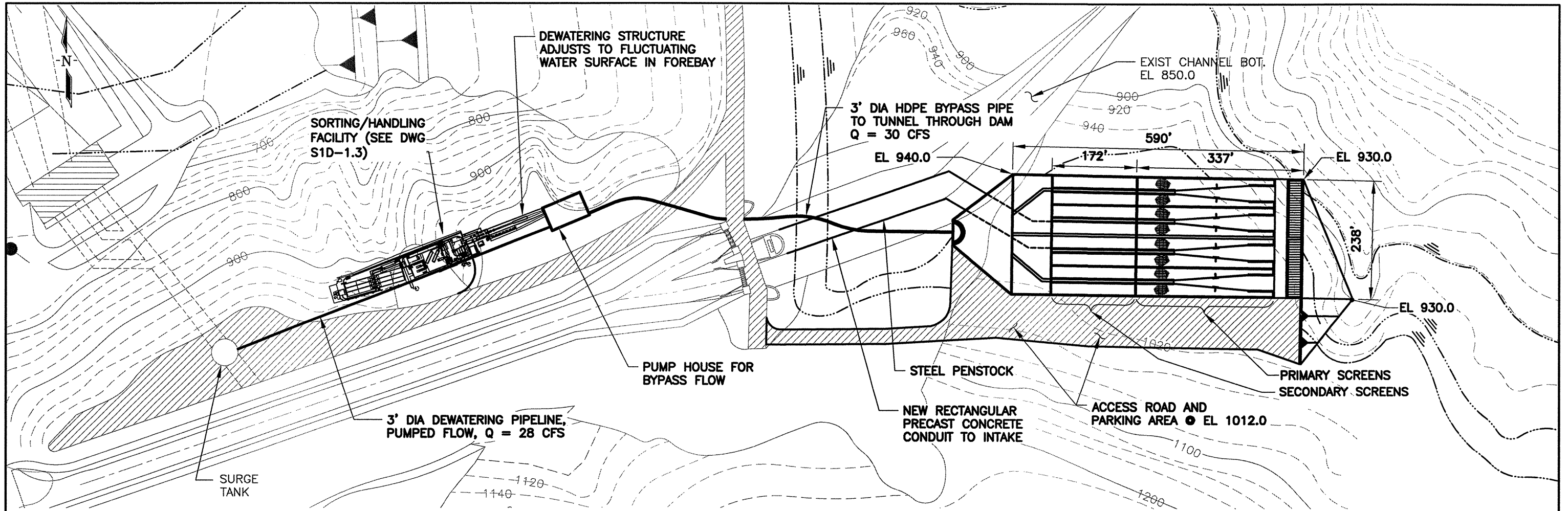
PLAN
