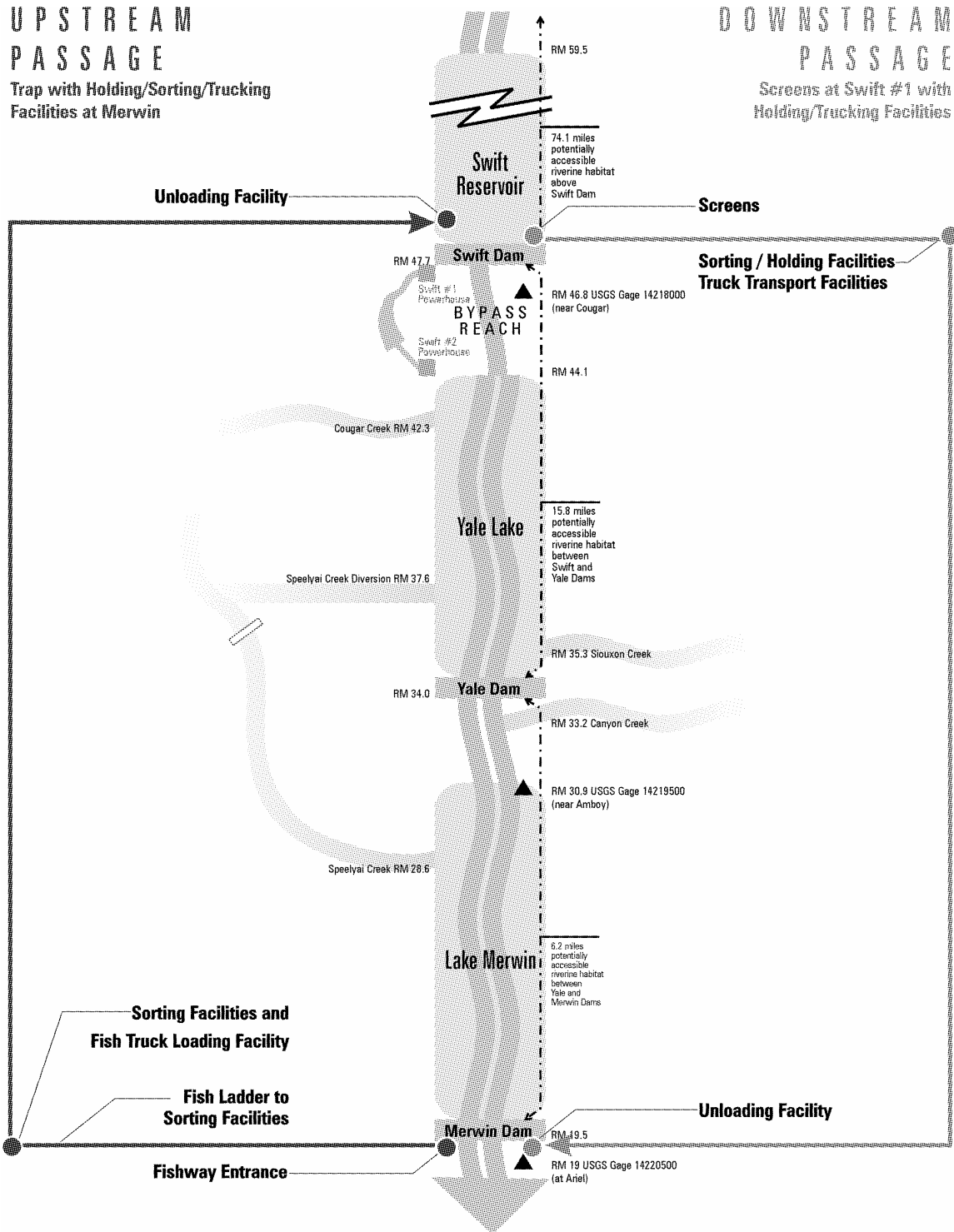
Figure 4.5-6. System 6: Trap-and-haul to upper Swift with screens (bypass Merwin and Yale).
