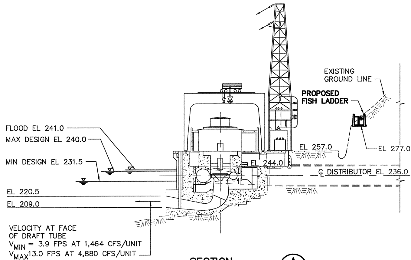
SECTION A APPROX STATION 5+00 YU-1.1
