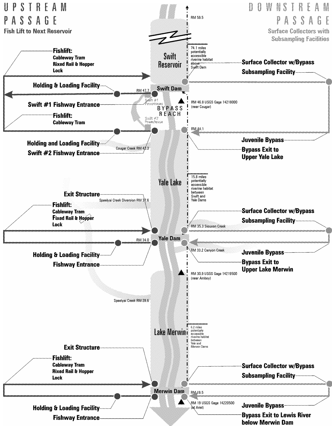
Figure 4.5-3. System 3: Fish lifts upstream, surface collectors downstream.
