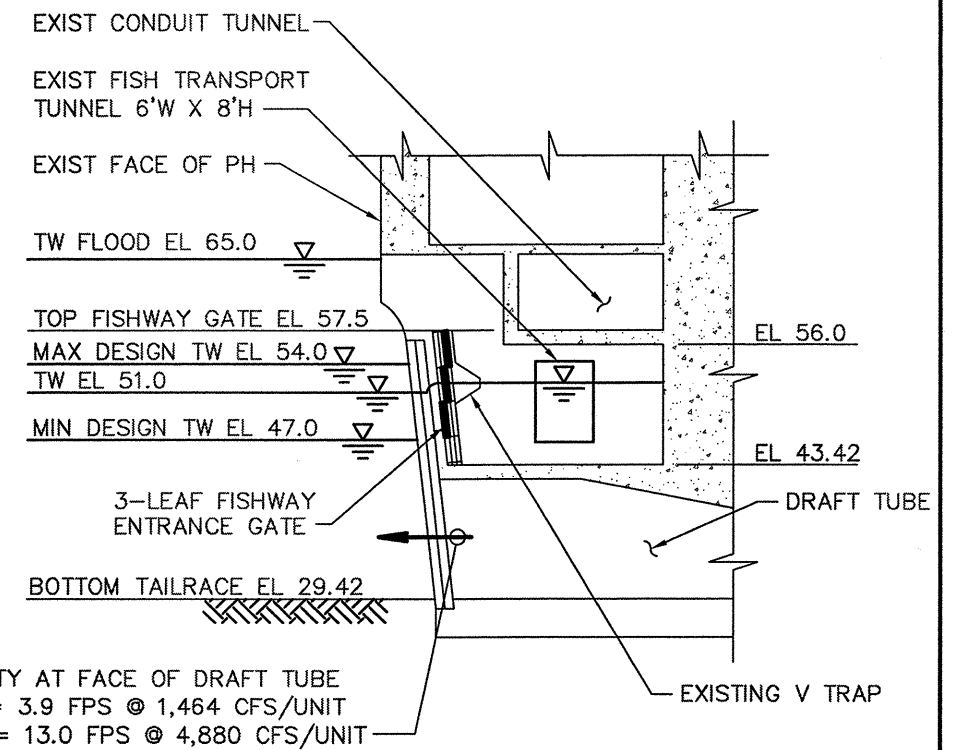
SECTION A-MU-2.2
