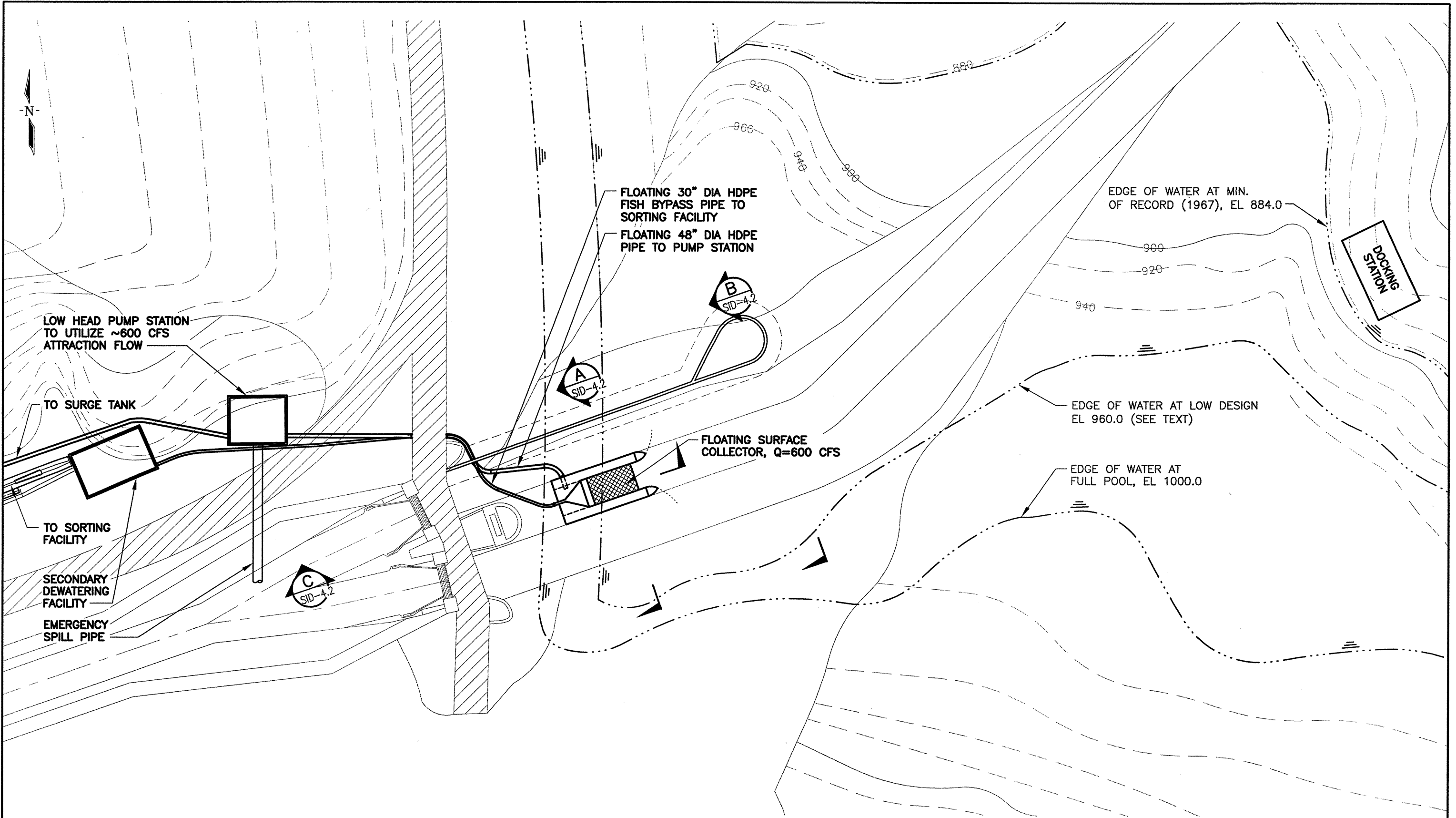
PLAN
