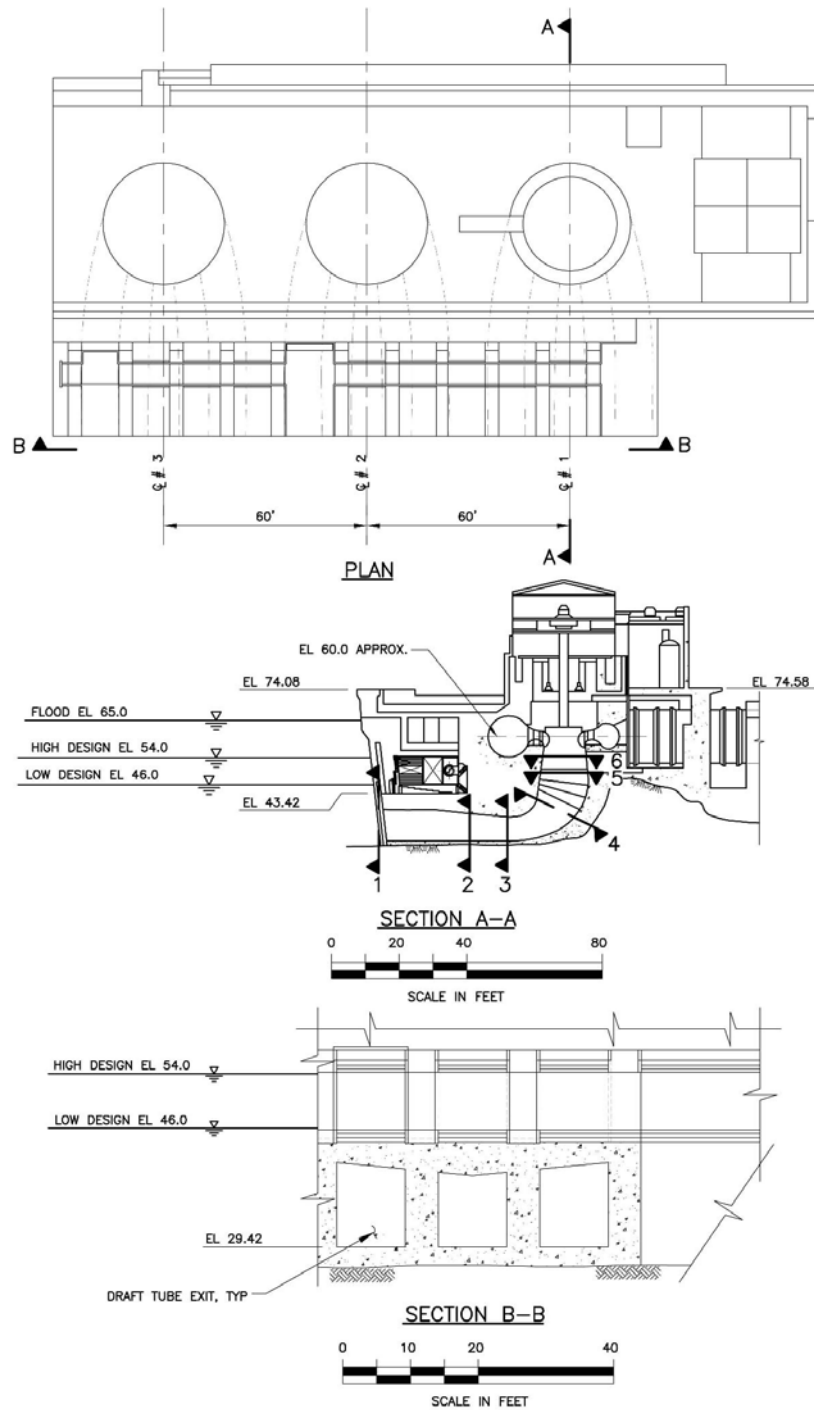
Figure 4.3-1. Merwin Dam draft tube configuration.
