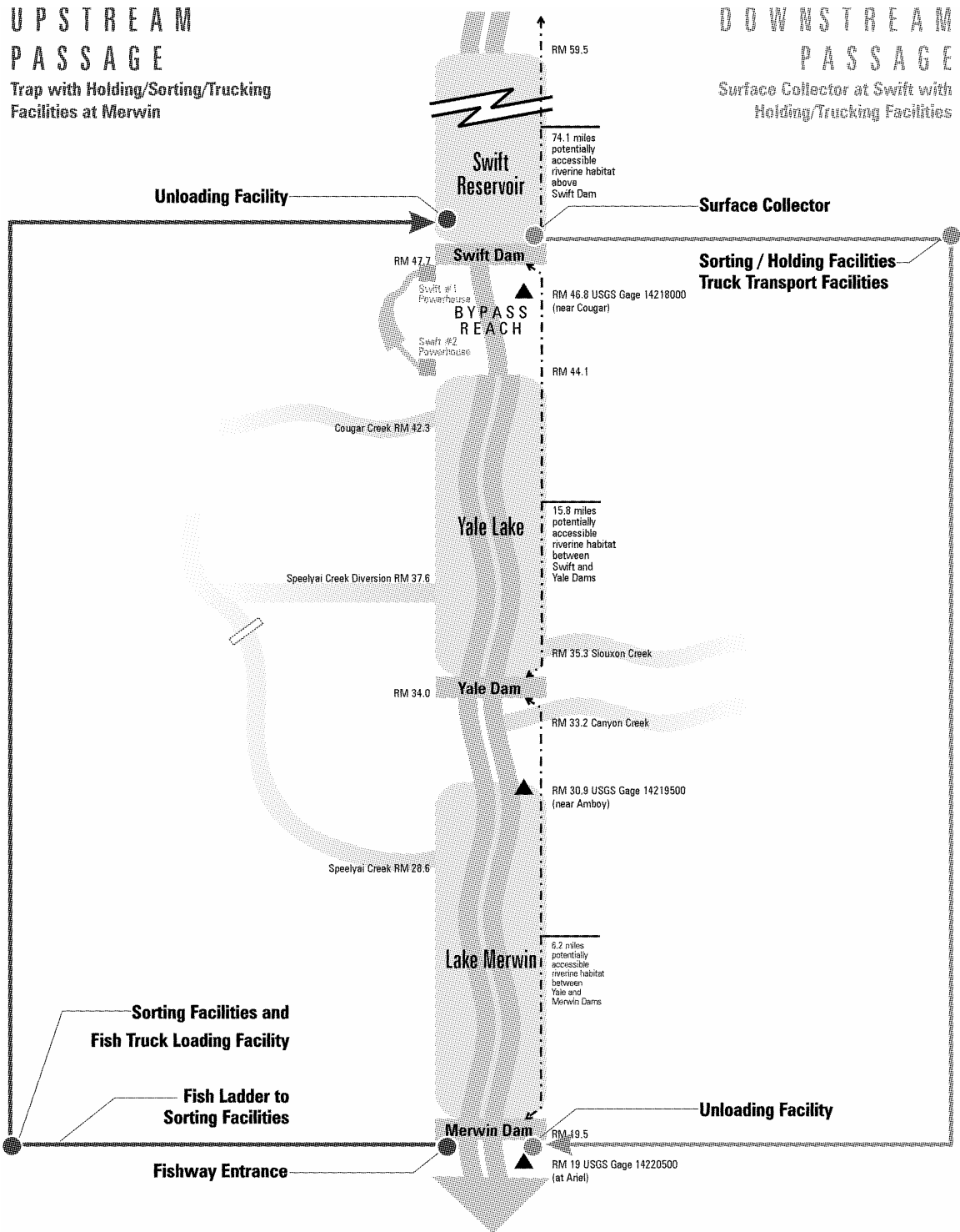
Figure 4.5-5. System 5: Trap-and-haul to upper Swift with surface collectors (bypass Merwin and Yale).
