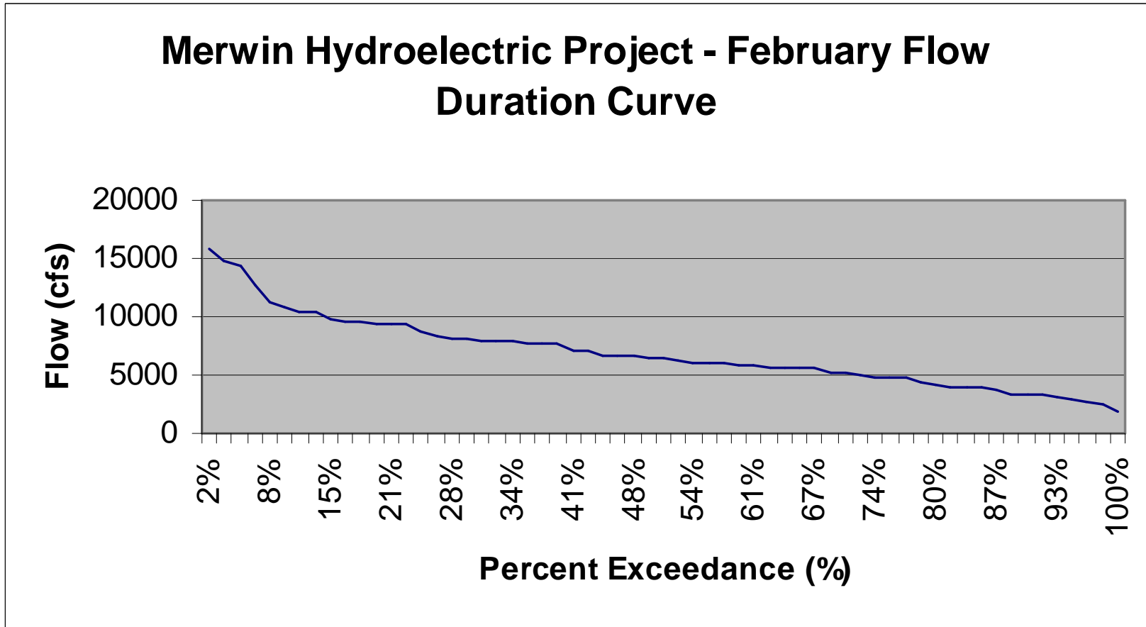
Merwin Flow Duration Curve – February
