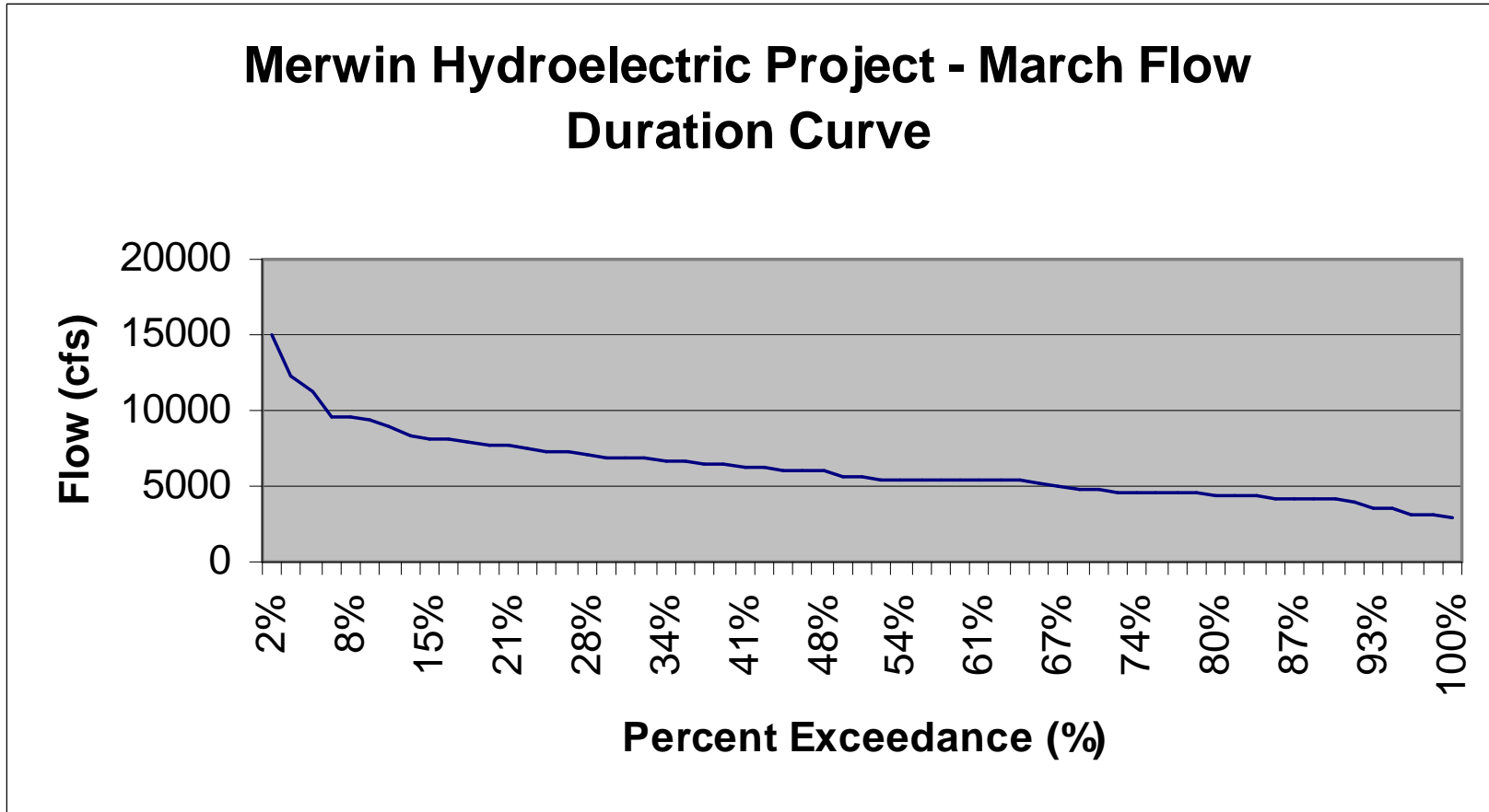
Merwin Flow Duration Curve – March
