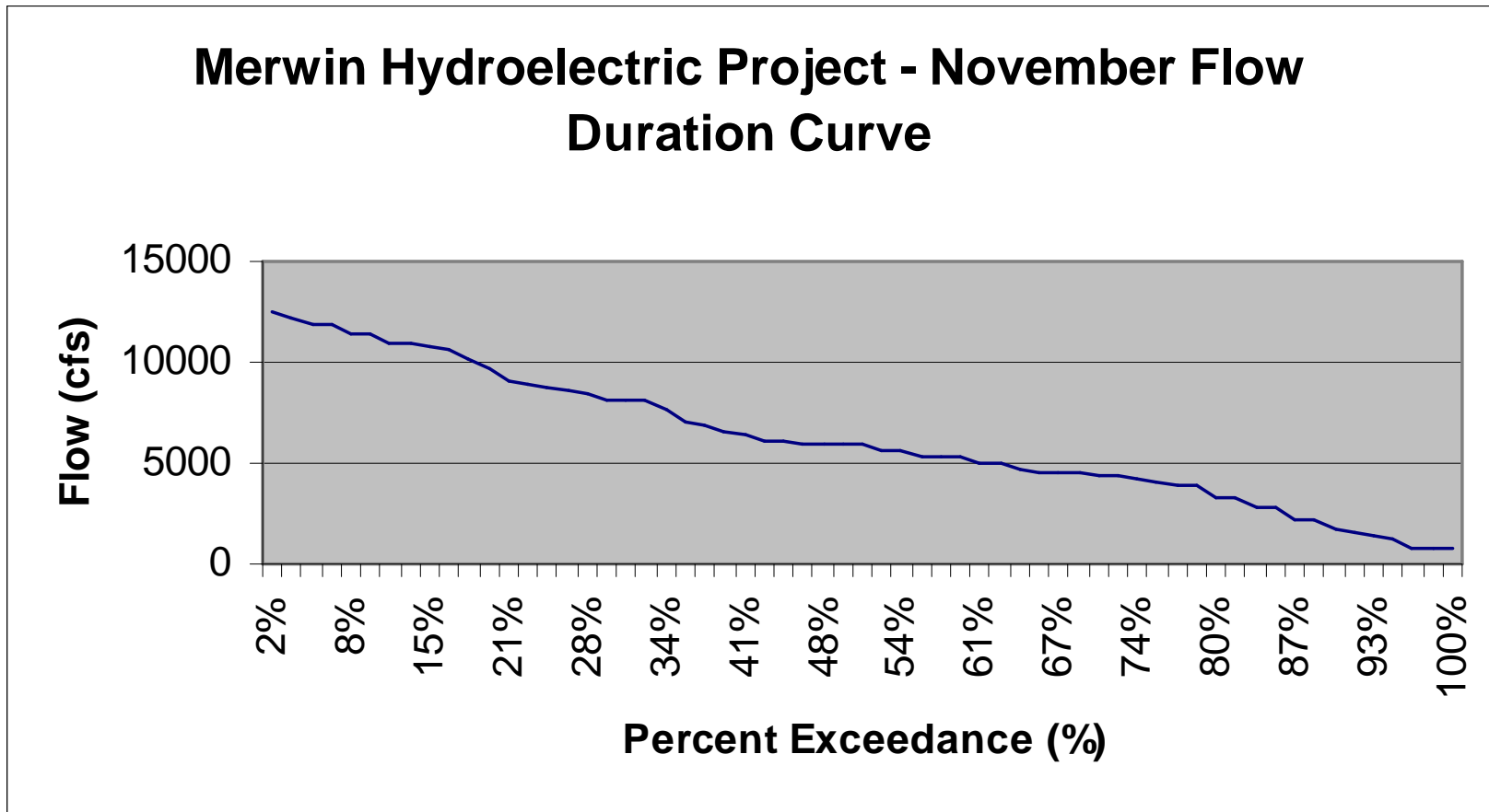
Merwin Flow Duration Curve – November
