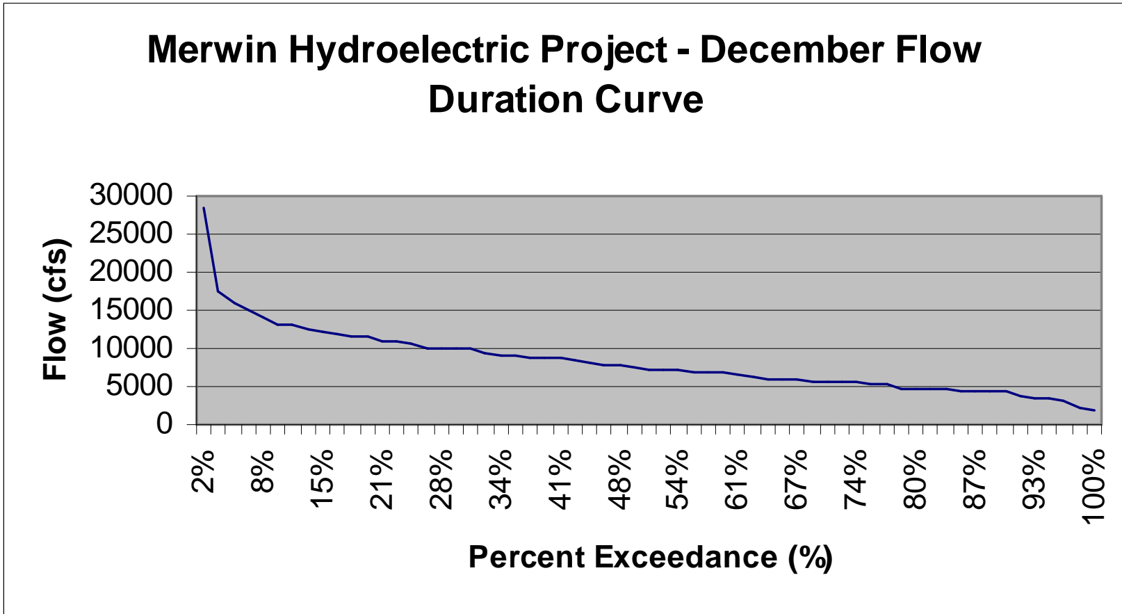
Merwin Flow Duration Curve – December
