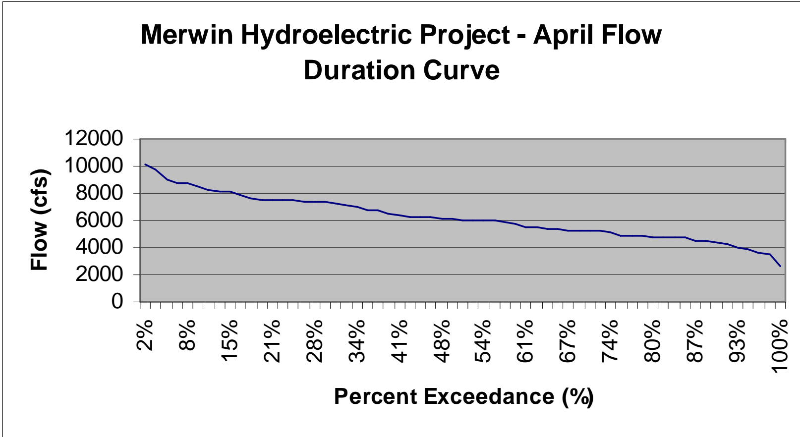
Merwin Flow Duration Curve – April
