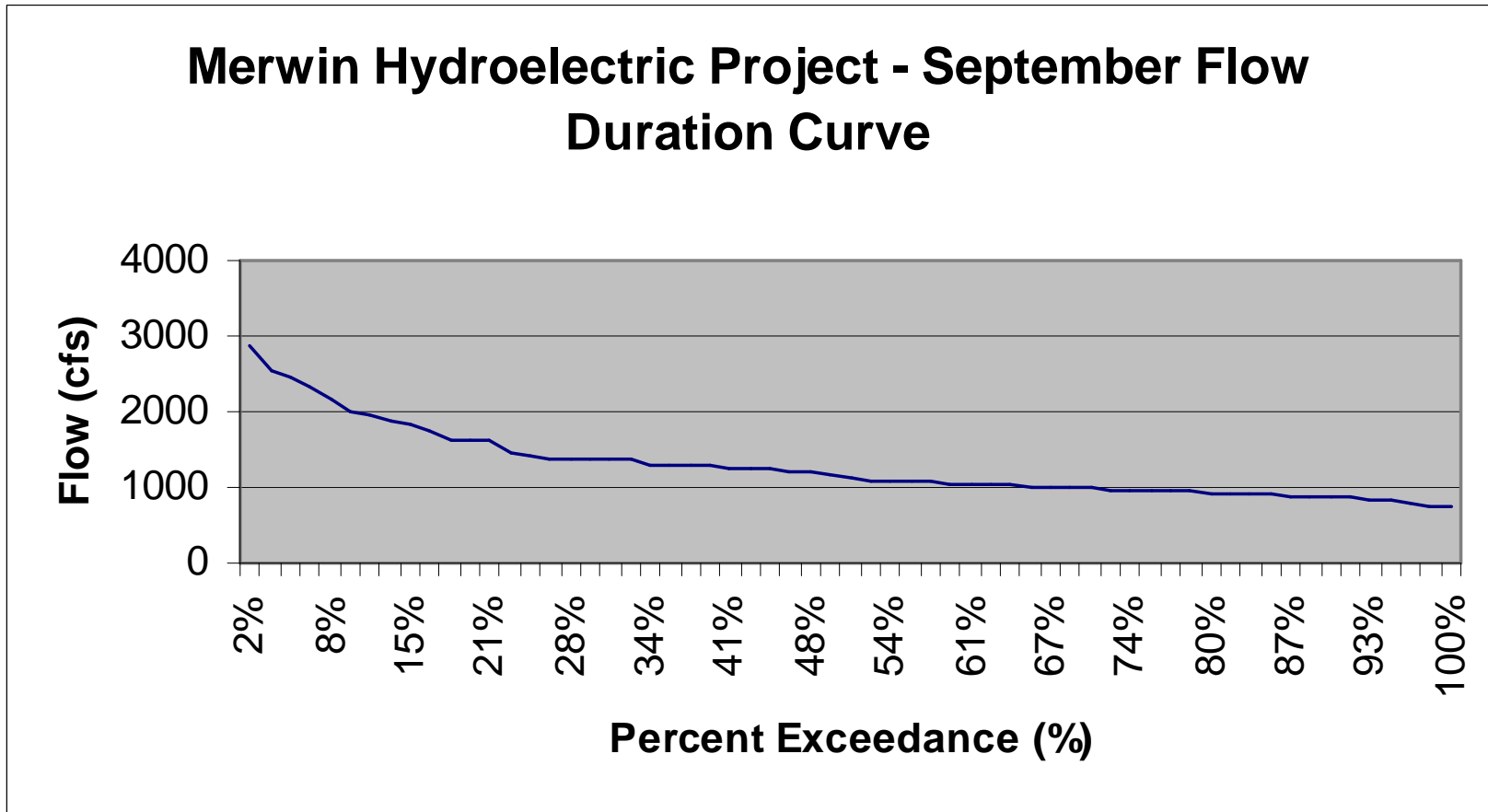
Merwin Flow Duration Curve – September
