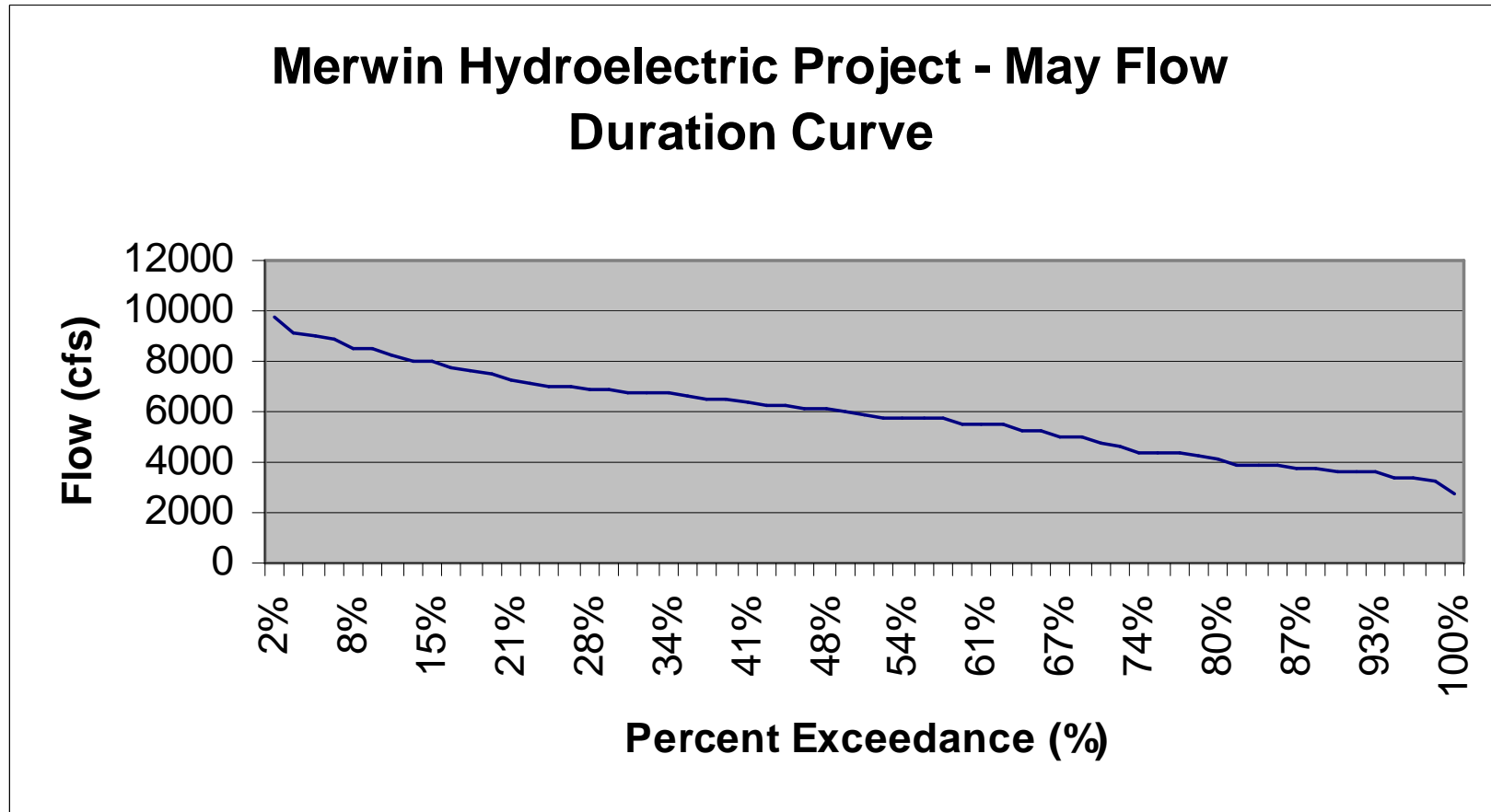
Merwin Flow Duration Curve – May
