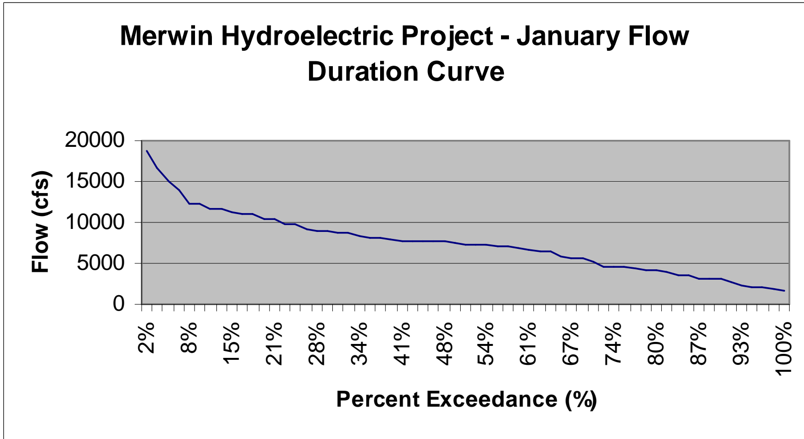
Merwin Flow Duration Curve – January
