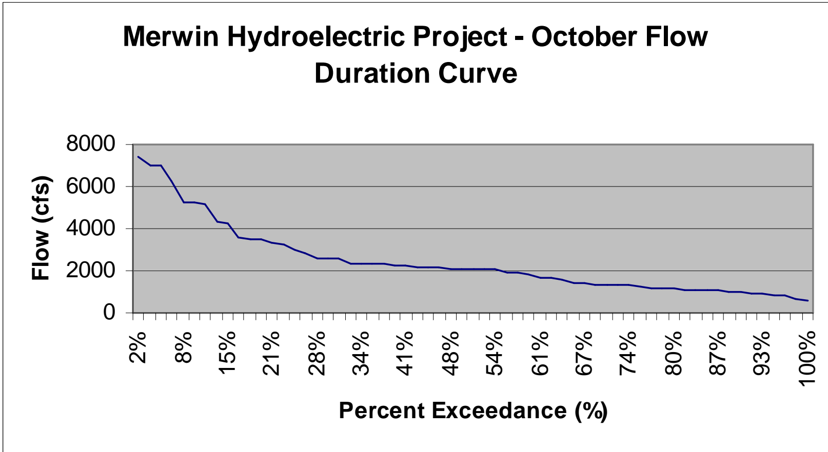
Merwin Flow Duration Curve – October
