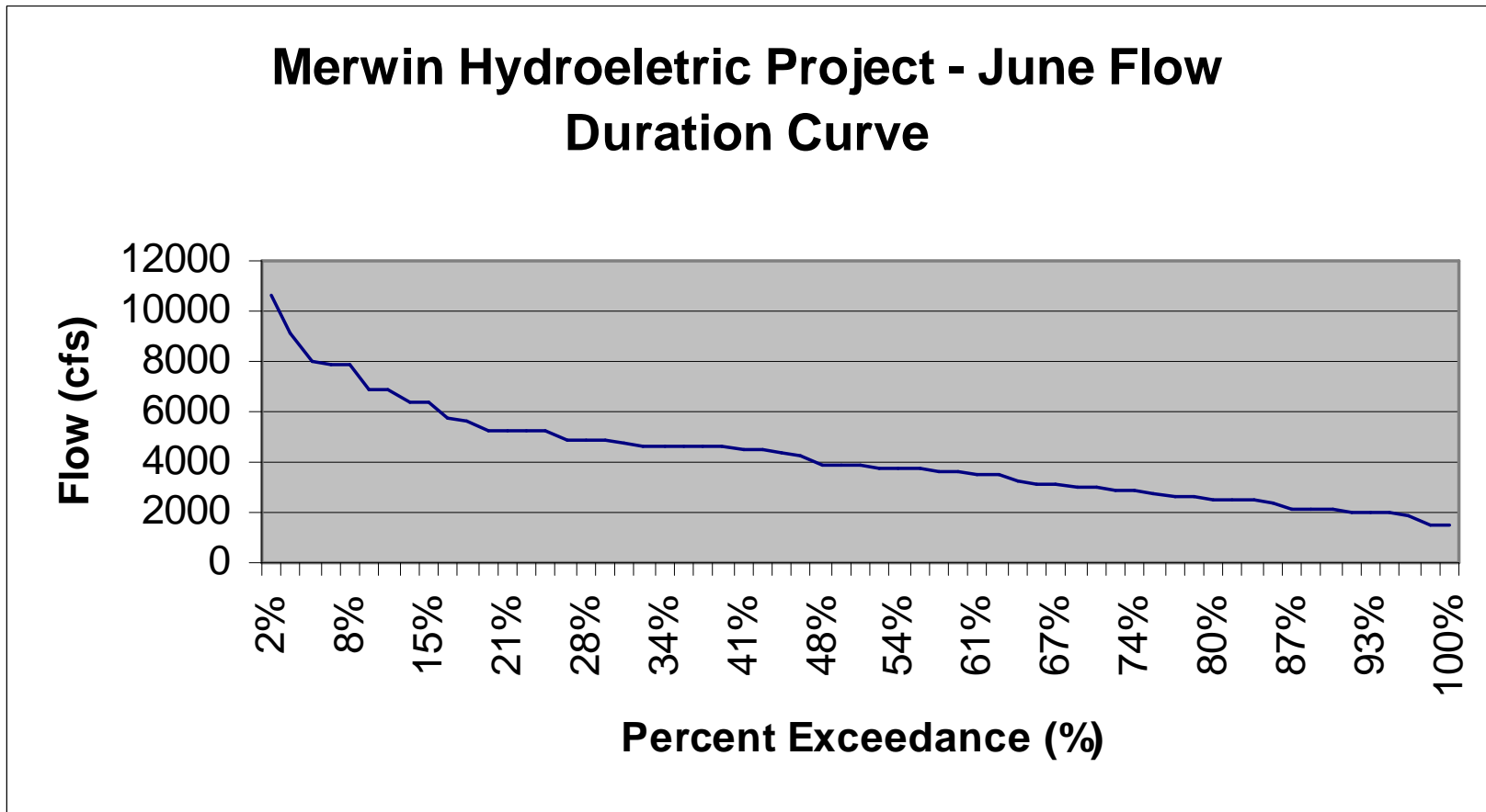
Merwin Flow Duration Curve – June
