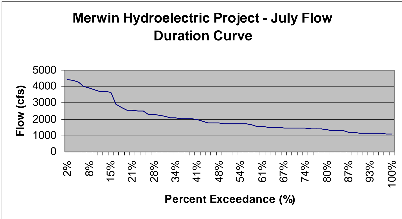
Merwin Flow Duration Curve – July
