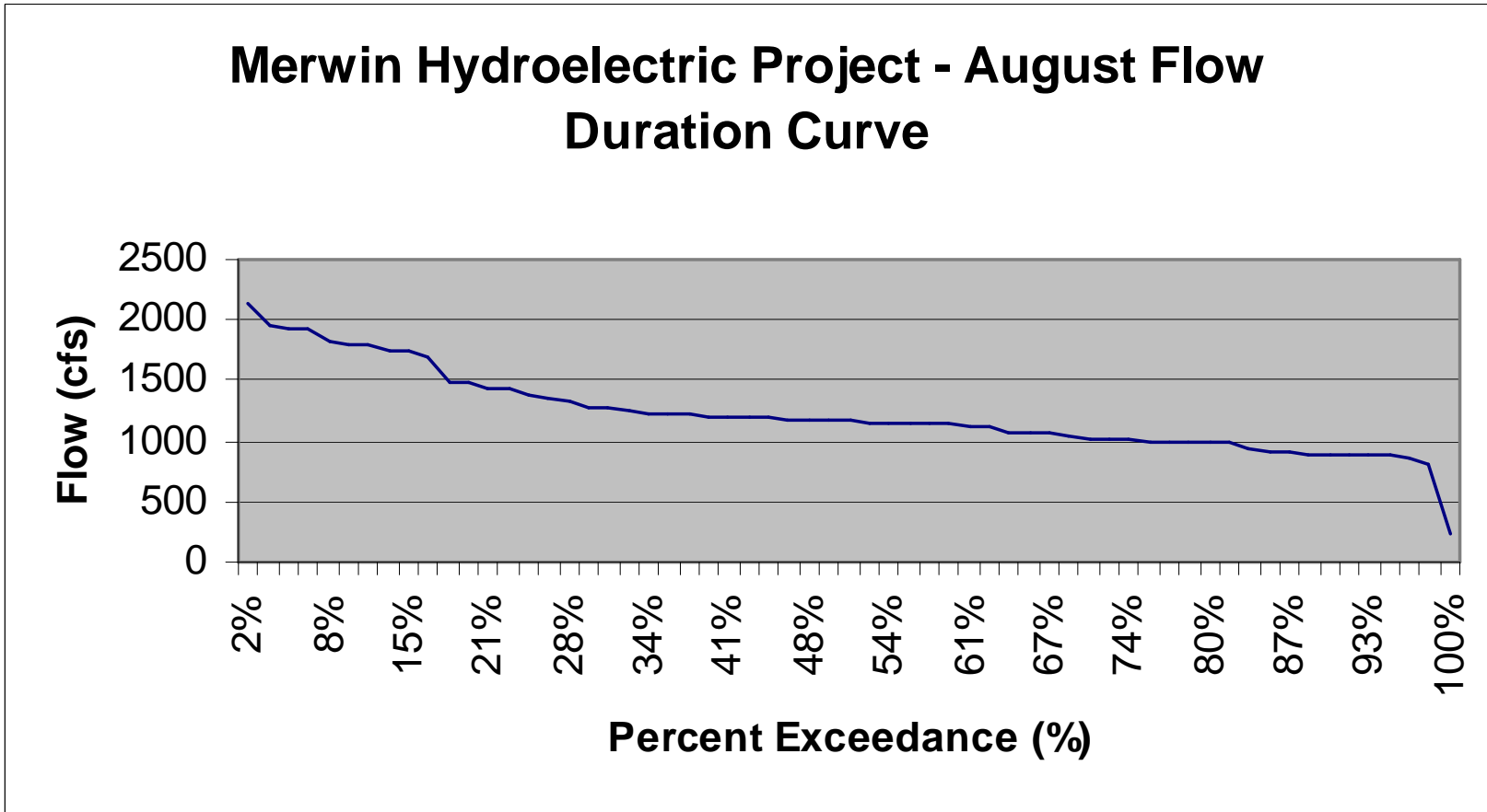
Merwin Flow Duration Curve – August
