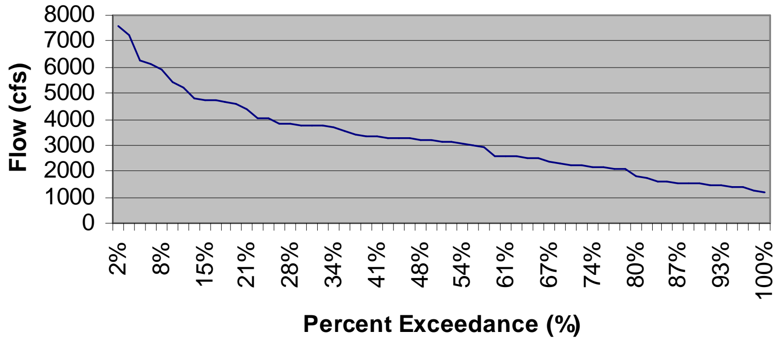
Swift No. 1 Flow Duration Curve – June
