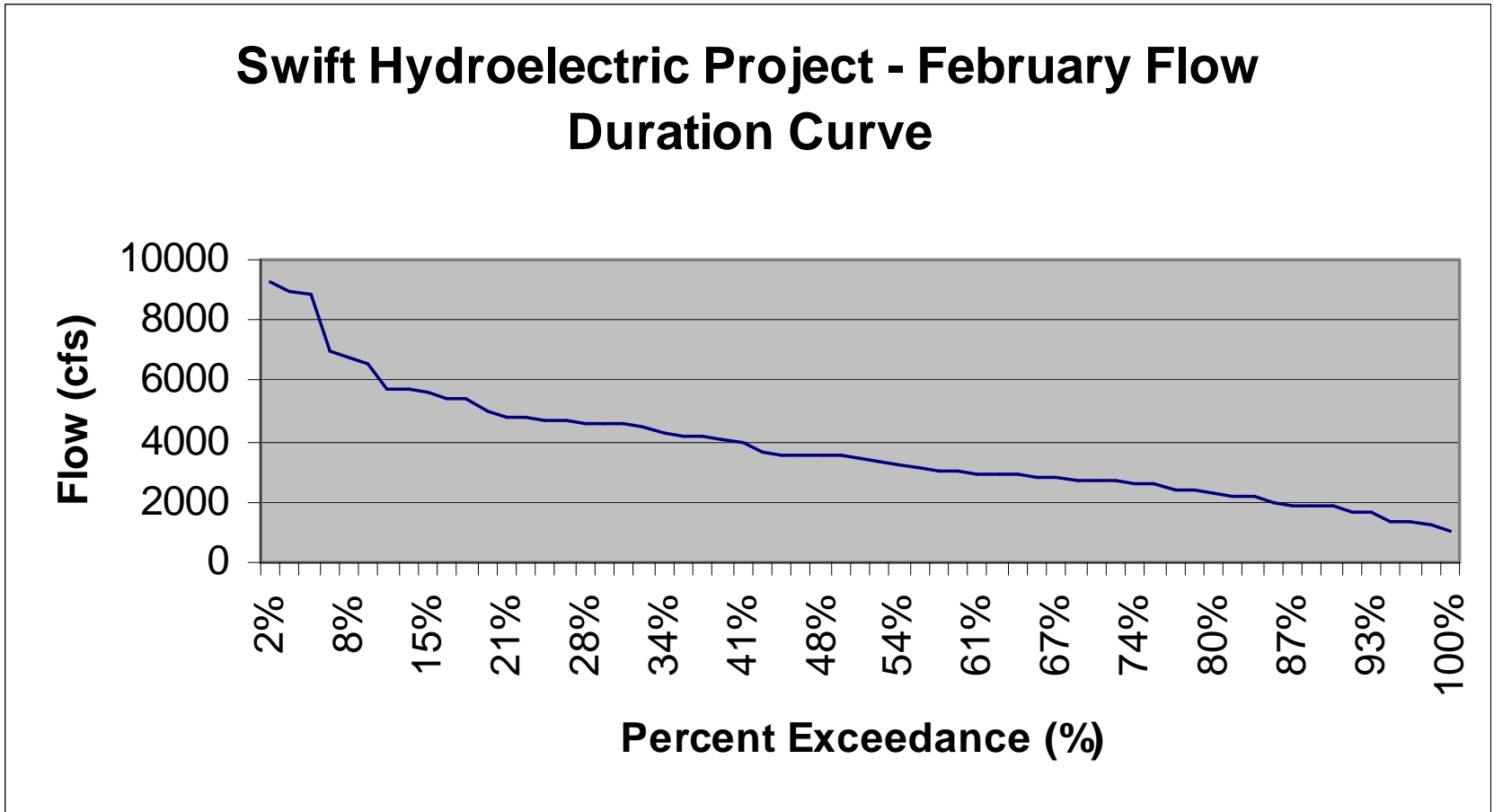
Swift No. 1 Flow Duration Curve – February
