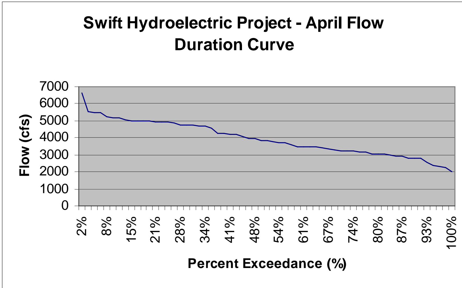
Swift No. 1 Flow Duration Curve – April
