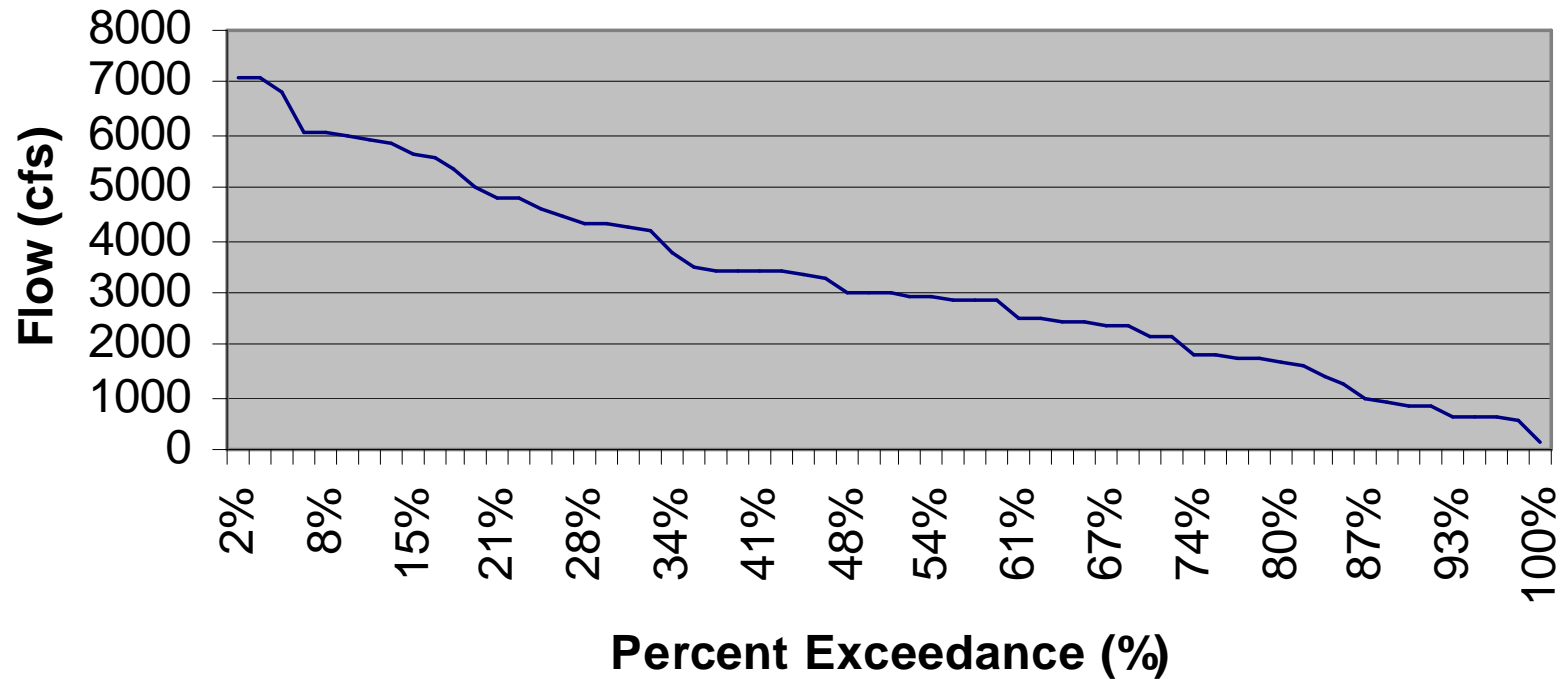
Swift No. 1 Flow Duration Curve – November
