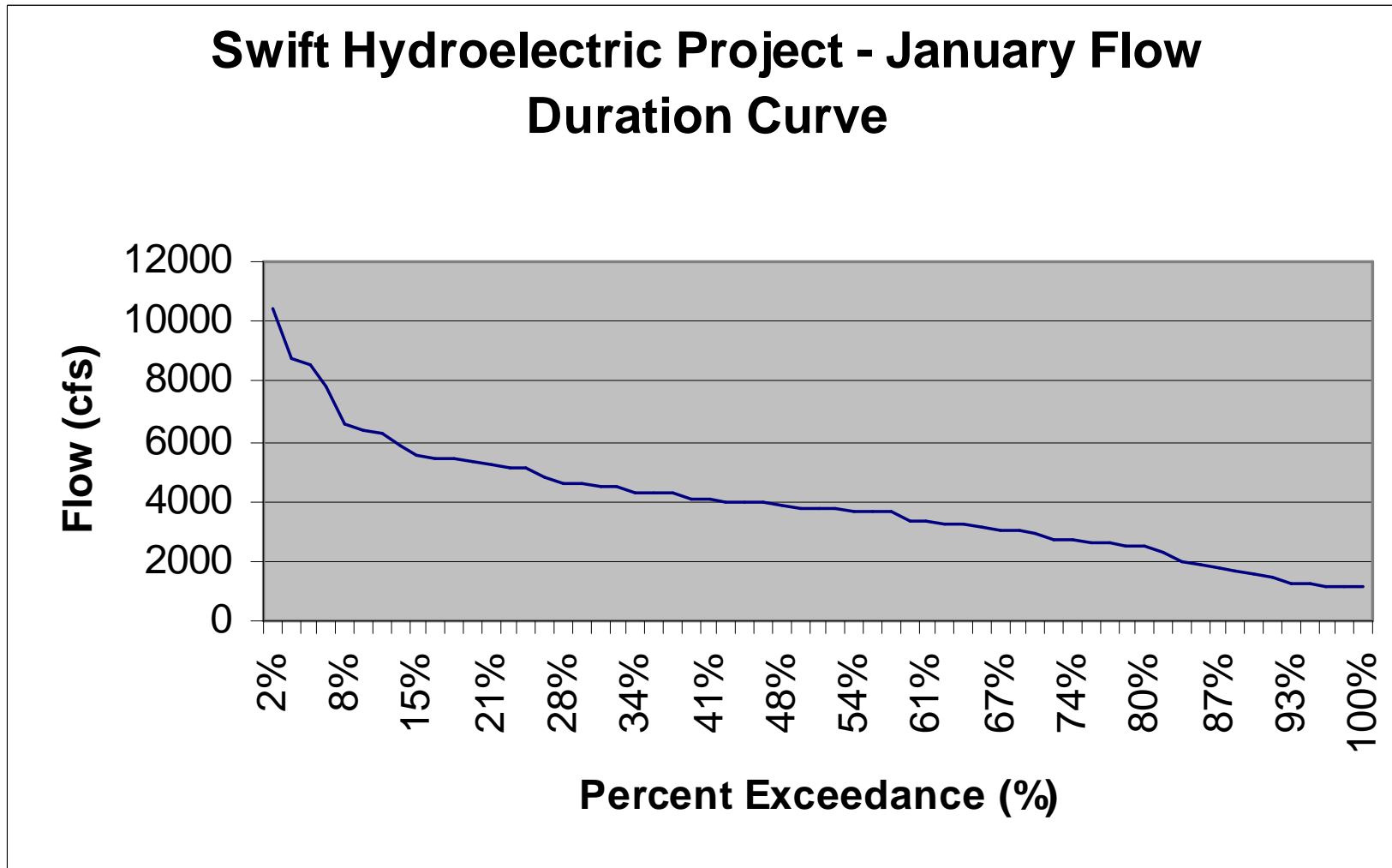
Swift No. 1 Flow Duration Curve – January
