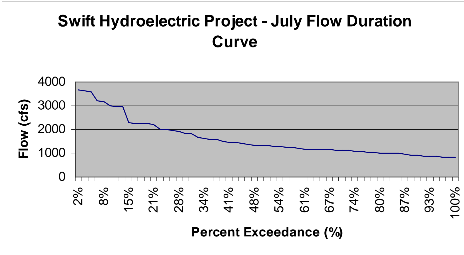
Swift No. 1 Flow Duration Curve – July
