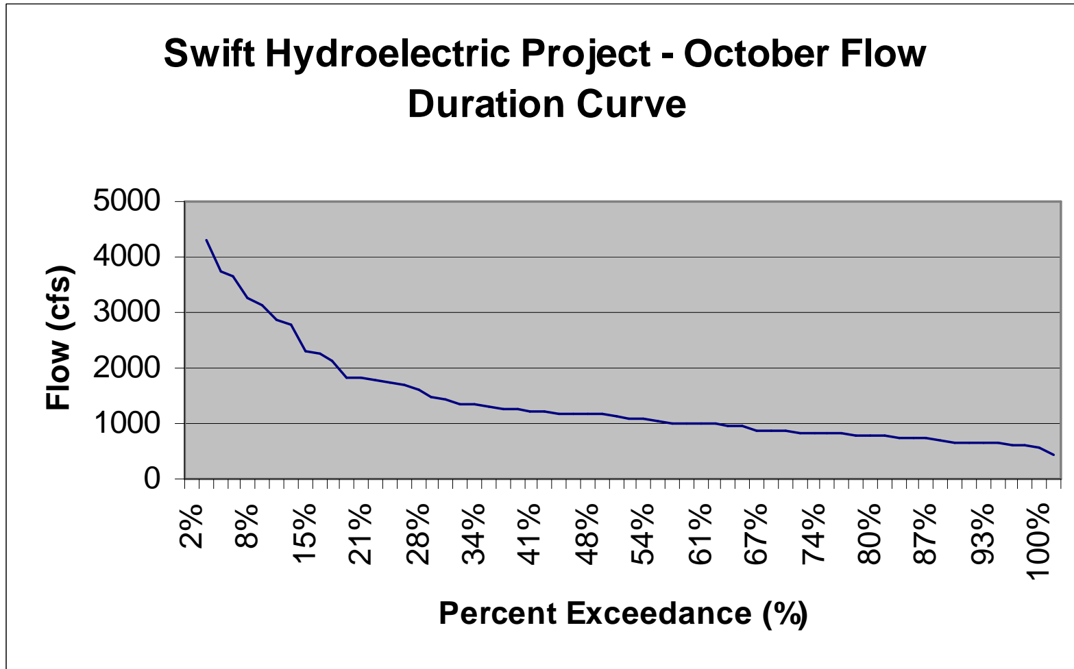
Swift No. 1 Flow Duration Curve – October
