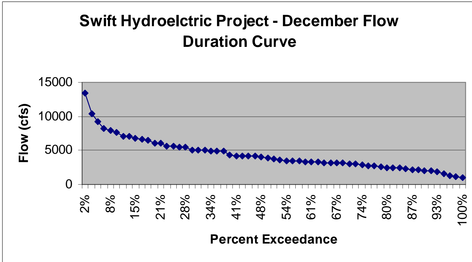
Swift No. 1 Flow Duration Curve – December
