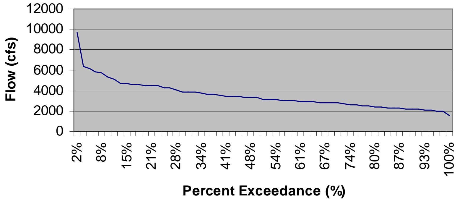
Swift No. 1 Flow Duration Curve – March
