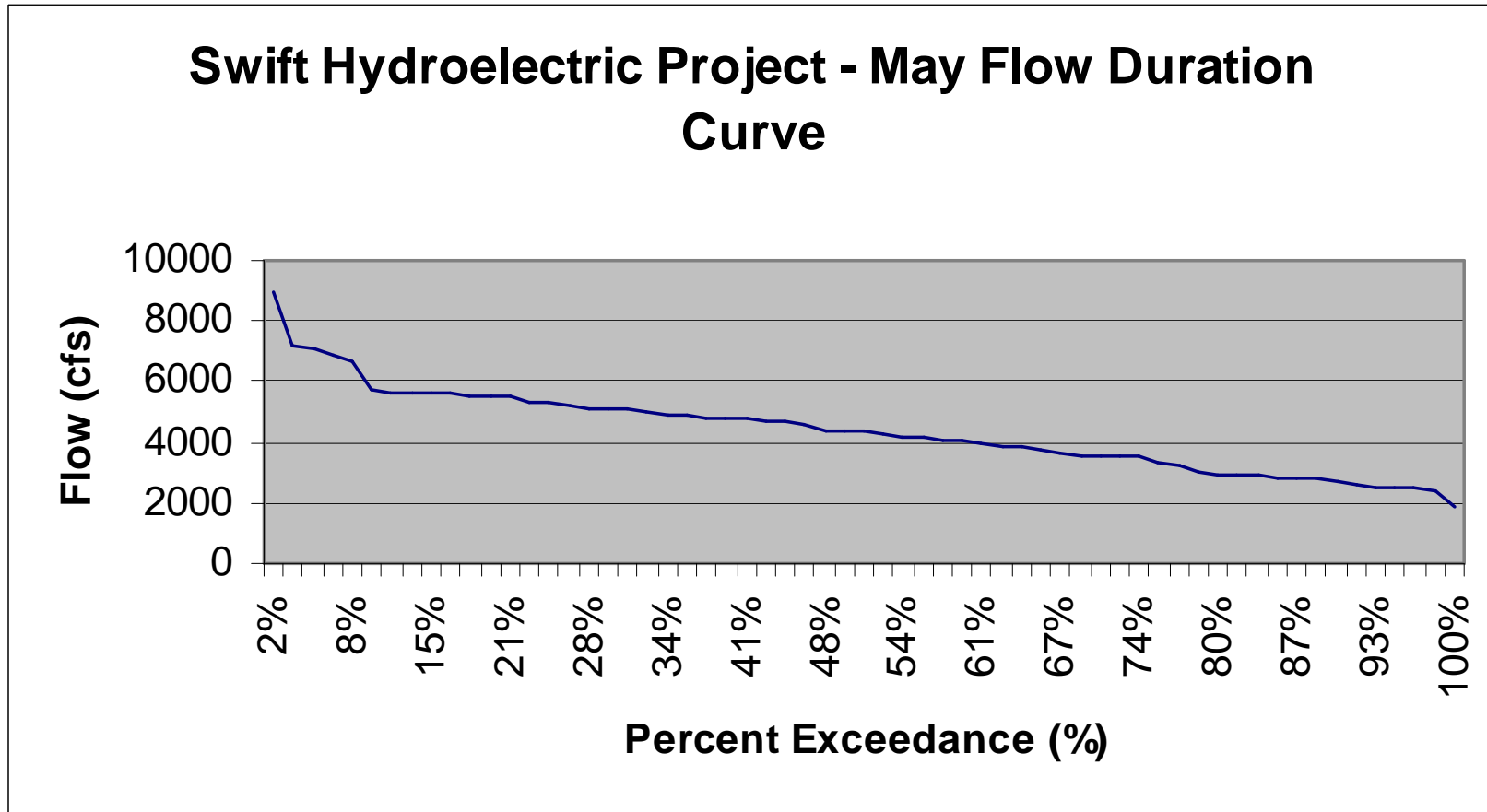
Swift No. 1 Flow Duration Curve – May
