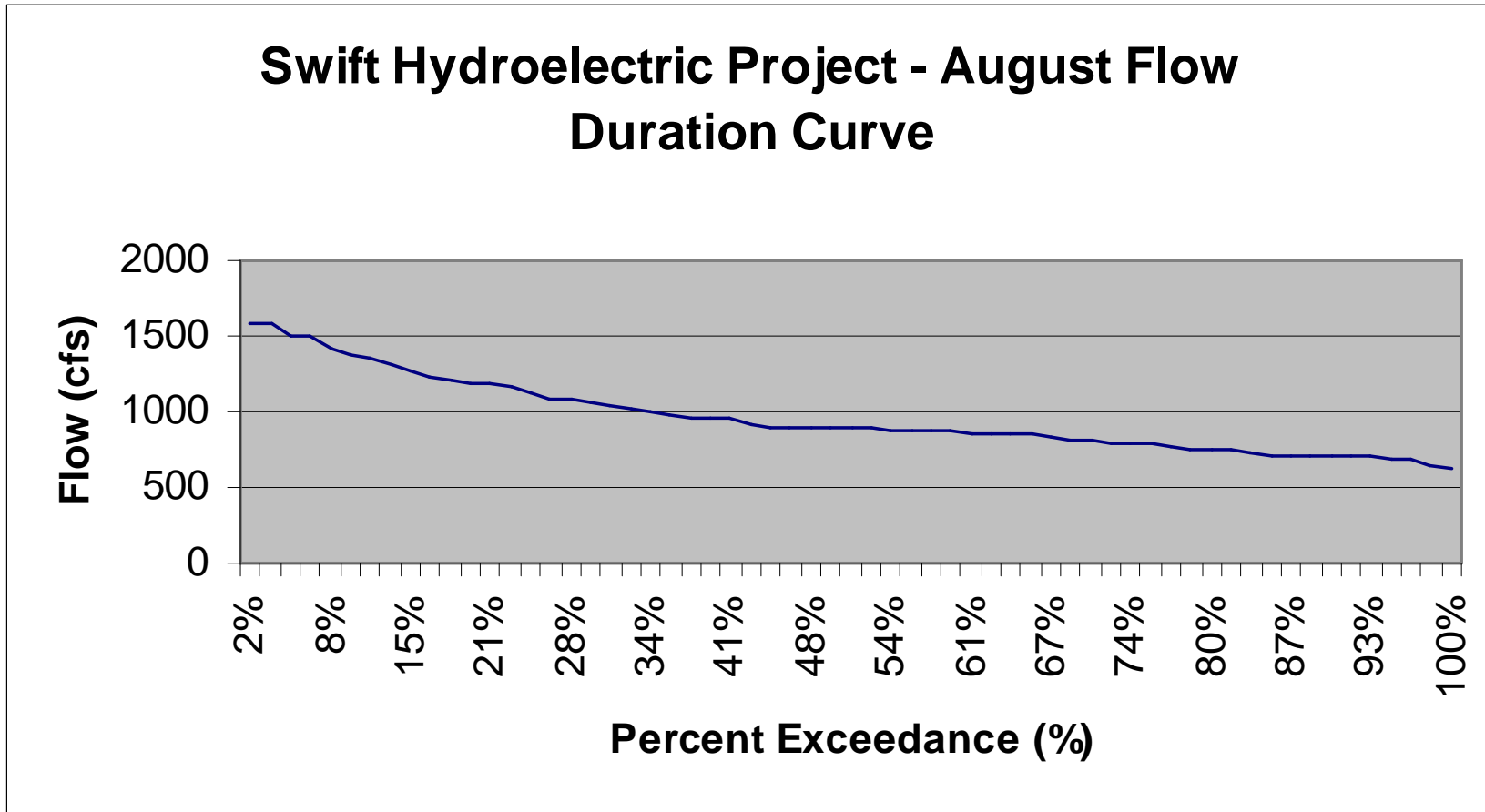
Swift No. 1 Flow Duration Curve – August
