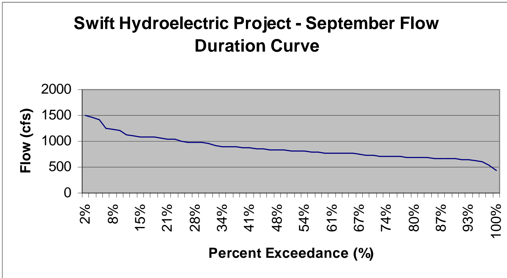
Swift No. 1 Flow Duration Curve – September
