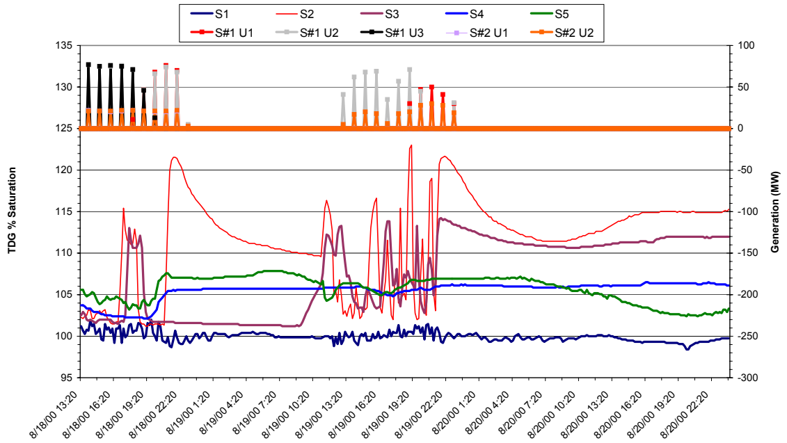
WAQ 2 Appendix 2 Figure 1. Total dissolved gas saturation values measured in Swift Power Canal, 18 to 27 August 2000.
