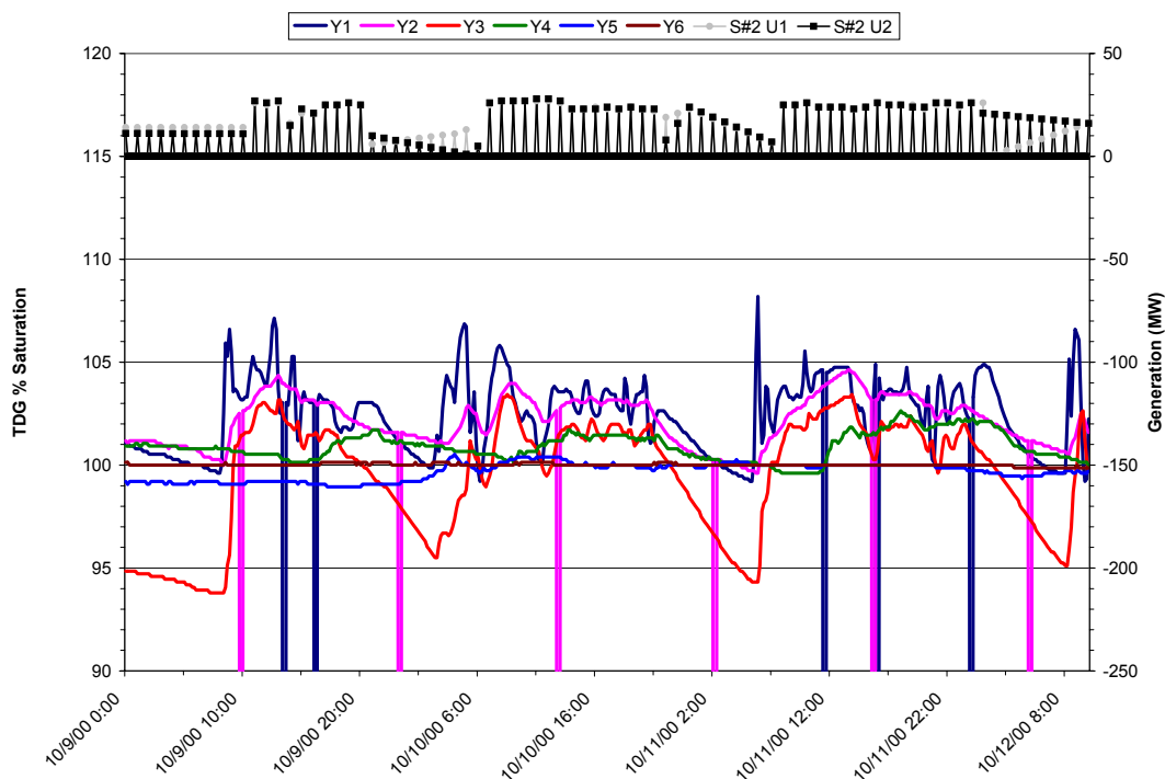
WAQ 2 Appendix 2 Figure 8. Total dissolved gas saturation values measured in Yale Lake, 9 to 12 October 2000.
