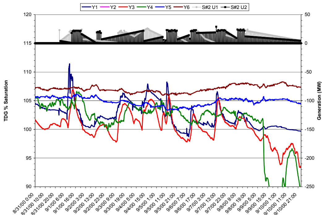
WAQ 2 Appendix 2 Figure 3. Total dissolved gas saturation values measured in Yale Lake for 31 August to 10 September 2000.
