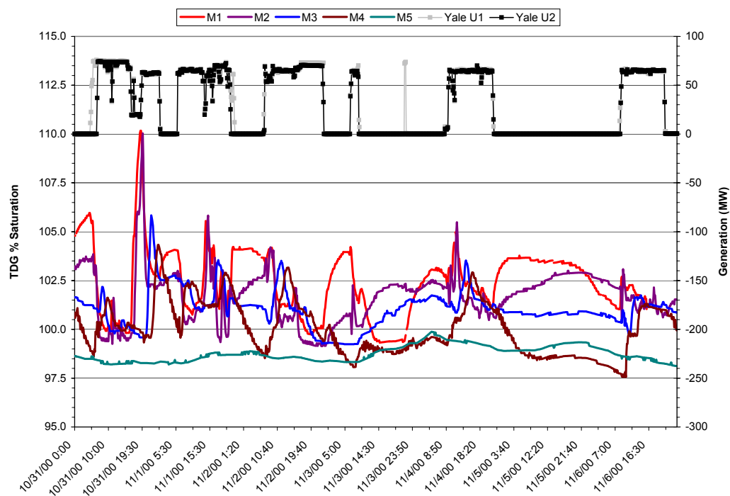
WAQ 2 Appendix 2 Figure 11. Total dissolved gas saturation values measured in Lake Merwin, 31 October to 6 November 2000.
