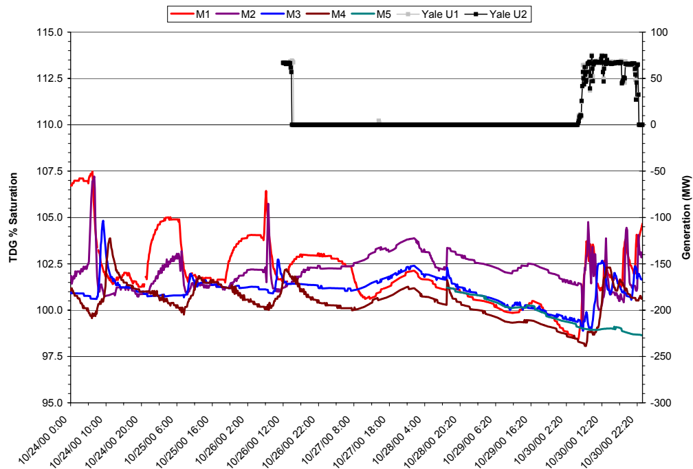
WAQ 2 Appendix 2 Figure 10. Total dissolved gas saturation values measured in Lake Merwin, 24 to 30 October 2000.
