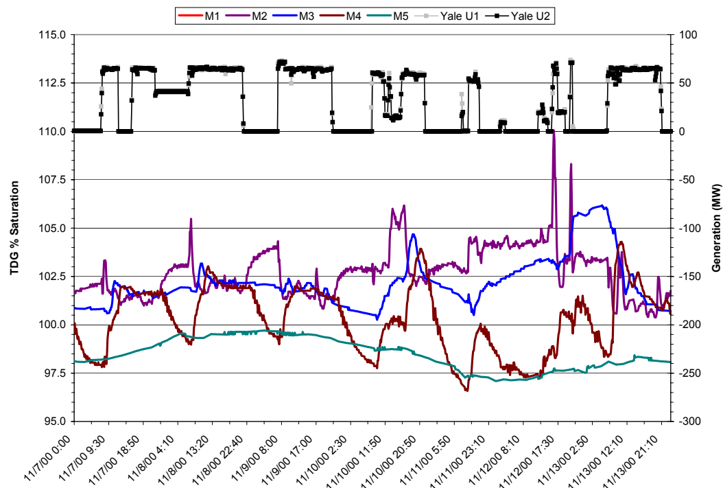
WAQ 2 Appendix 2 Figure 12. Total dissolved gas saturation values measured in Lake Merwin, 7 to 13 November 2000.
