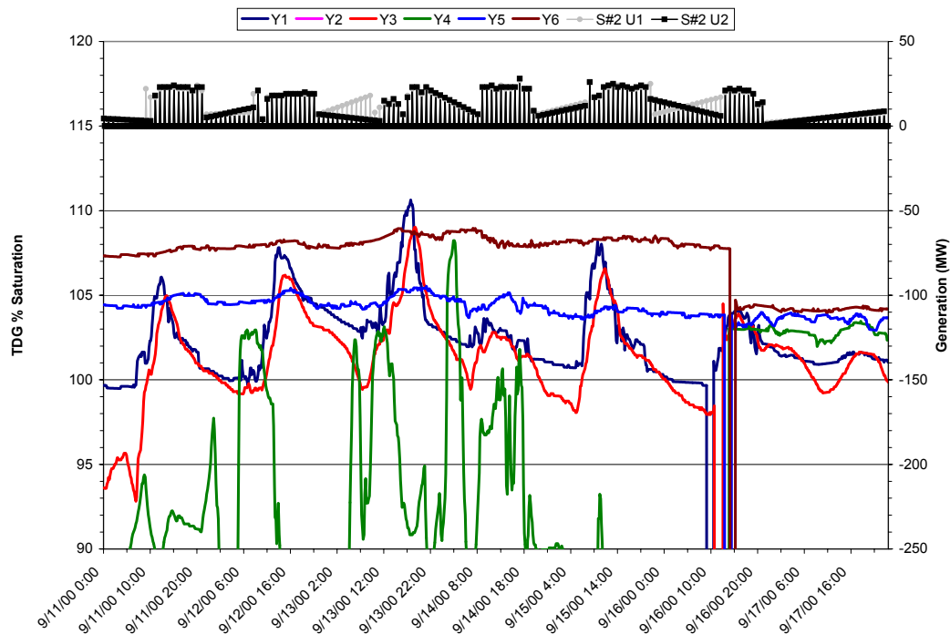
WAQ 2 Appendix 2 Figure 4. Total dissolved gas saturation values measured in Yale Lake for 11 to 17 September 2000.
