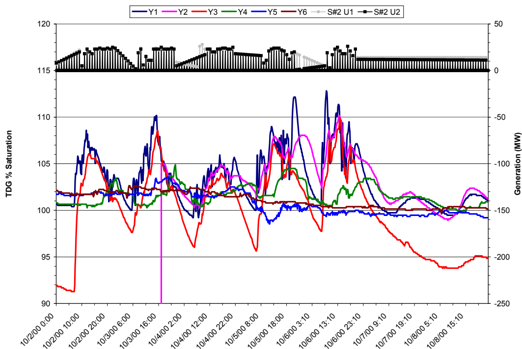
WAQ 2 Appendix 2 Figure 7. Total dissolved gas saturation values measured in Yale Lake, 2 to 8 October 2000.
