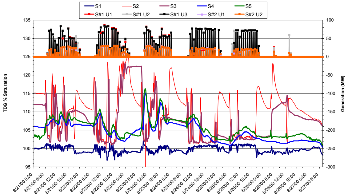
WAQ 2 Appendix 2 Figure 2. Total dissolved gas saturation values measured in Swift Power Canal, 21 to 27 August 2000.
