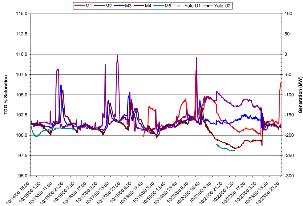
WAQ 2 Appendix 2 Figure 9. Total dissolved gas saturation values measured in Lake Merwin, 14 to 23 October 2000.
