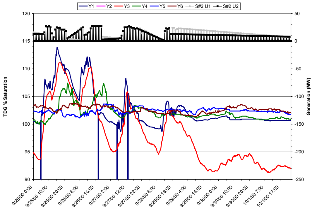
WAQ 2 Appendix 2 Figure 6. Total dissolved gas saturation values measured in Yale Lake, 25 September to 1 October 2000.
