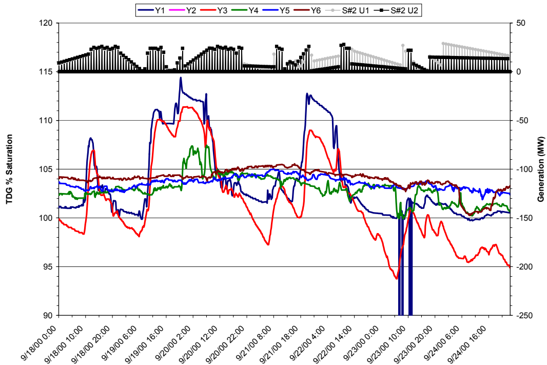
WAQ 2 Appendix 2 Figure 5. Total dissolved gas saturation values measured in Yale Lake, 18 to 24 September 2000.
