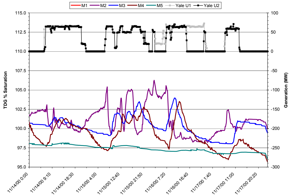
WAQ 2 Appendix 2 Figure 13. Total dissolved gas saturation values measured in Lake Merwin, 14 to 17 November 2000.
