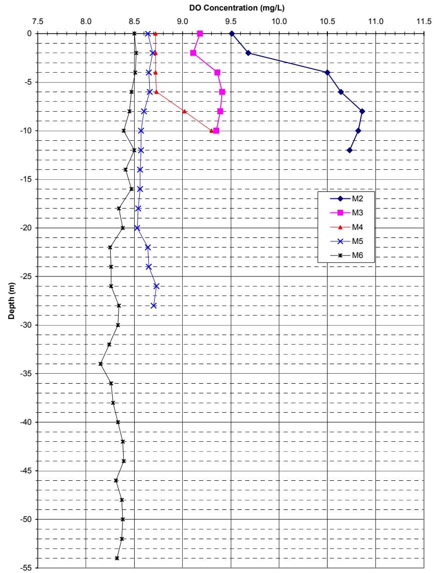
WAQ2 Appendix 3. Figure 6. Temperature and dissolved oxygen profiles for Lake Merwin, 21 October 2000.
