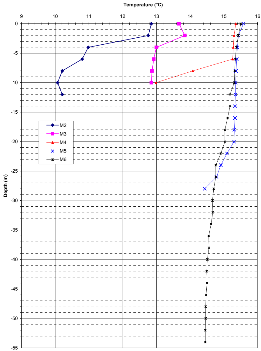
WAQ2 Appendix 3. Figure 6. Temperature and dissolved oxygen profiles for Lake Merwin, 21 October 2000.
