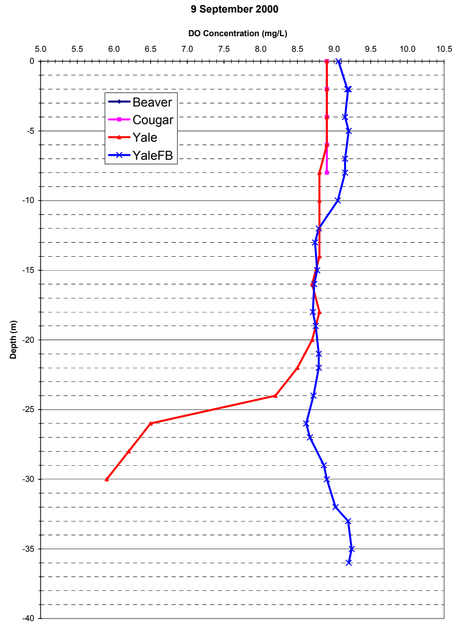
WAQ2 Appendix 3. Figure 2. Temperature and dissolved oxygen profiles for Yale Lake, 9 September 2000.
