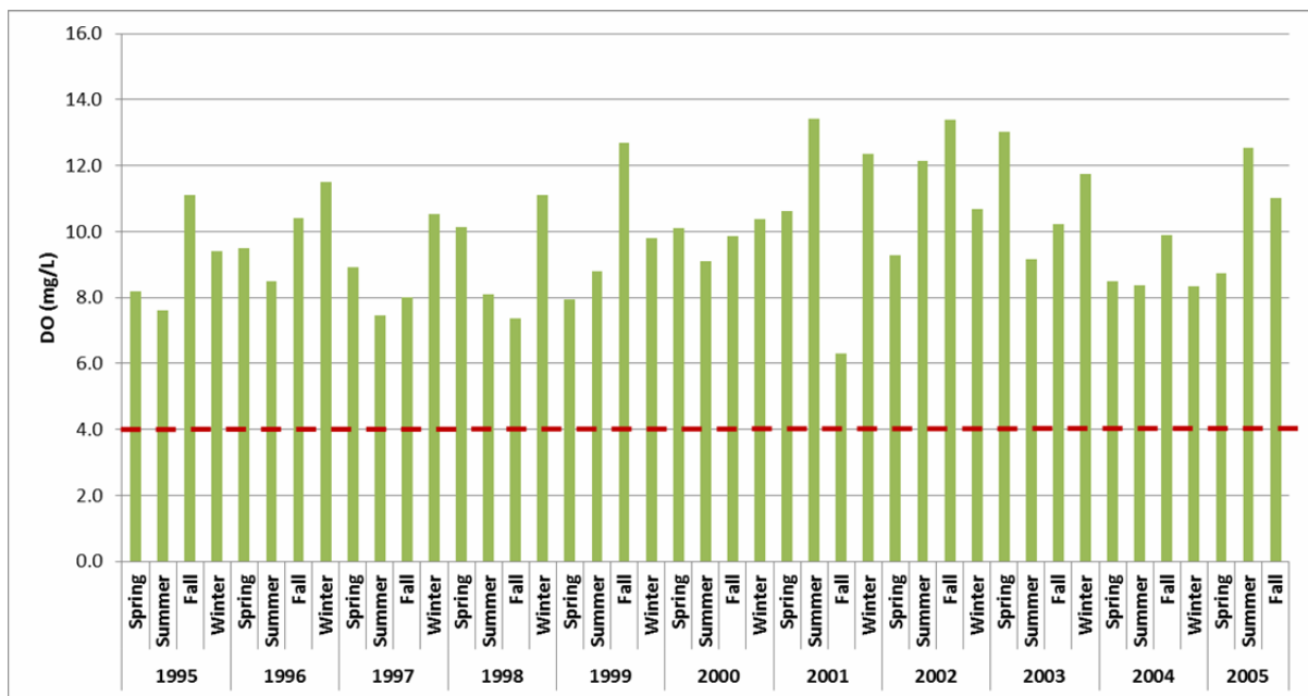
Figure 4. Minimum DO values by season from 1995 to 2005 compared to the UDEQ DO standard of 4.0 mg/L as a 1-day minimum (red dashed line) for Class 3A waters.
