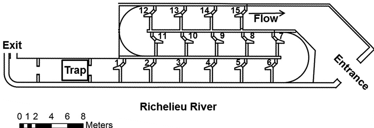
Figure 1. Schematic of the fishway showing the fishway entrance and exit, the location of the fish trap, the flow direction, and each basin labeled with its corresponding passive integrated transponder antenna number.
