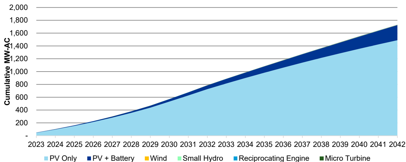
Figure 4-22 Cumulative New Capacity Installed by Technology (MW-AC), Utah Base Case, 2023-2042
