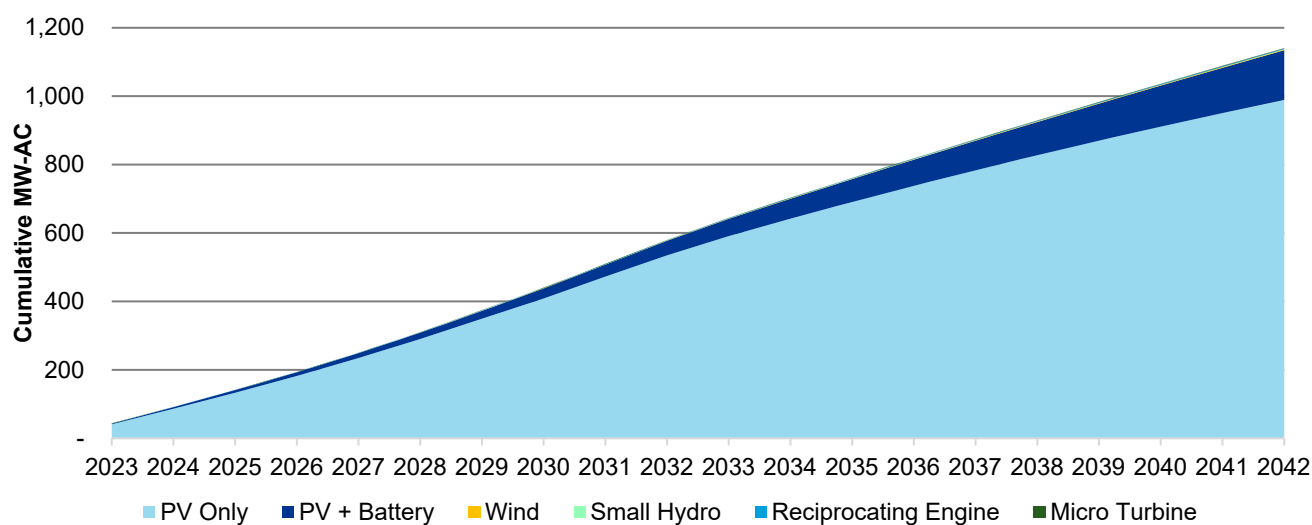
Figure 4-23 Cumulative New Capacity Installed by Technology (MW-AC), Utah Low Case, 2023-2042
