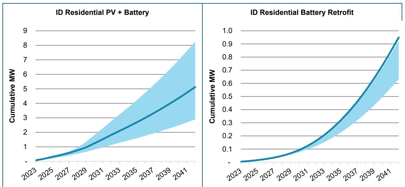
Figure E-12 Cumulative New Battery Storage Capacity Installed by Technology Across All Scenarios (MW), Idaho, 2023-2042
