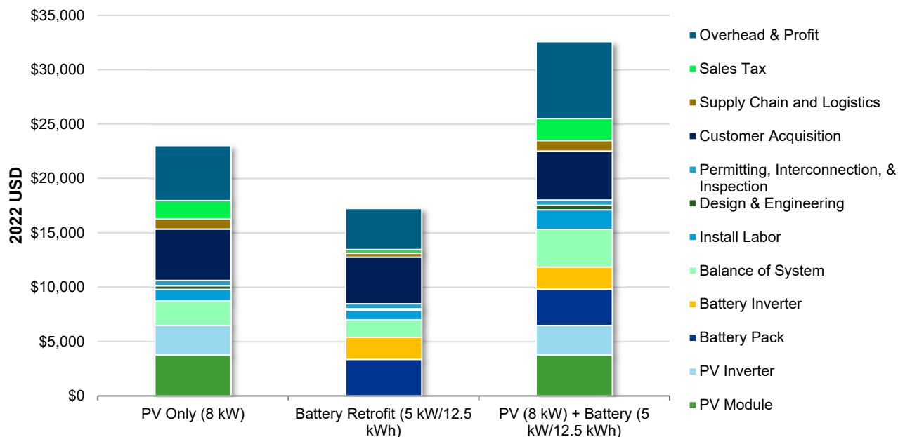
Figure 3-3 Cost of Commercial PV Standalone, Battery Storage Retrofit to Existing PV, and PV + Battery Systems from DNV Bottom-up Cap-Ex Model, Utah
