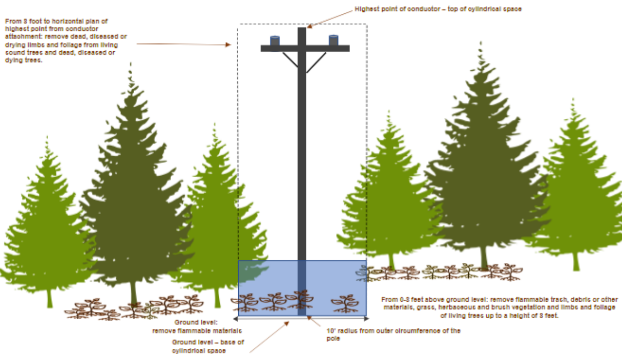
Figure 8-12 Pole Clearing
